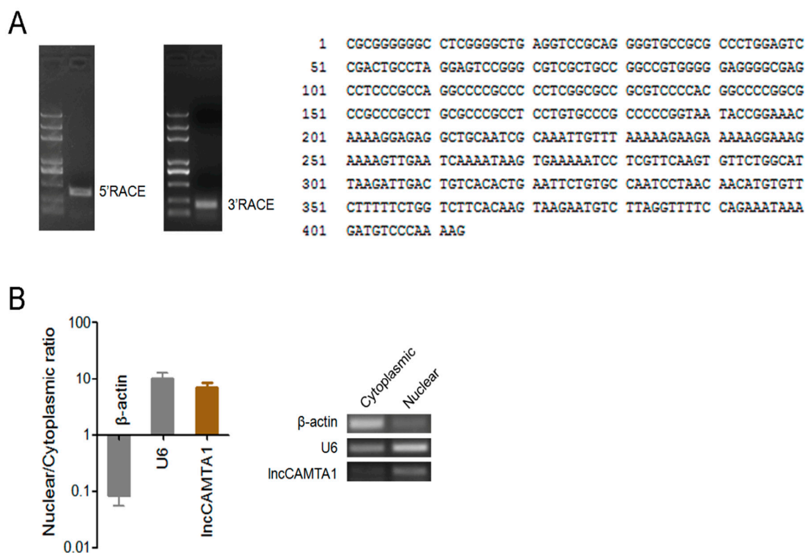
Figure S1. Full-length sequences and subcellular localization of lncCAMTA1 in hepatocellular carcinoma cells. (A) Full-length nucleotide sequences of lncCAMTA1; (B) Quantitative real-time PCR (qRT-PCR) analysis of lncCAMTA1 subcellular location in HCCLM3 cells. \beta -actin and U6 were used as cytoplasmic and nuclear markers respectively. n = 3 .
