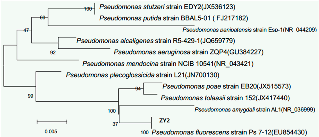
Figure S1. The phylogenetic tree of the strain named ZY2.
