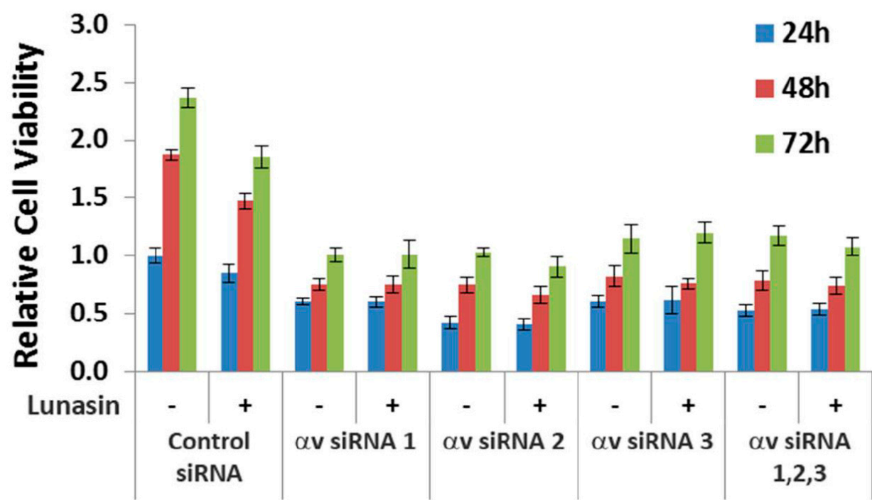
Figure S1. Proliferation of control siRNA transfected H661 cells transfected with a control siRNA or three different siRNAs designed to silence \alpha v expression individually or in combination. Proliferation assays were initiated 48 h after transfection with siRNAs; cells were treated with either 50 mM sodium phosphate buffer (vehicle) or 100 \mu M lunasin. Data shown are the mean \pm SD obtained in three independent experiments.
