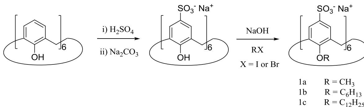
Figure 2. Synthesis of alkylated p -sulfonatocalix[6]arenes.
