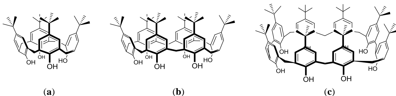
Figure 1. Structures of tert -butylcalix[ n ]arenes. (a) n = 4 ; (b) n = 6 ; (c) n = 8 .
