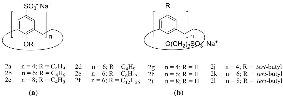
Figure 3. Amphiphilic sulfonatocalix[ n ]arenes bearing the hydrophilic SO 3 - group at the (a) upper rim and (b) lower rim.
