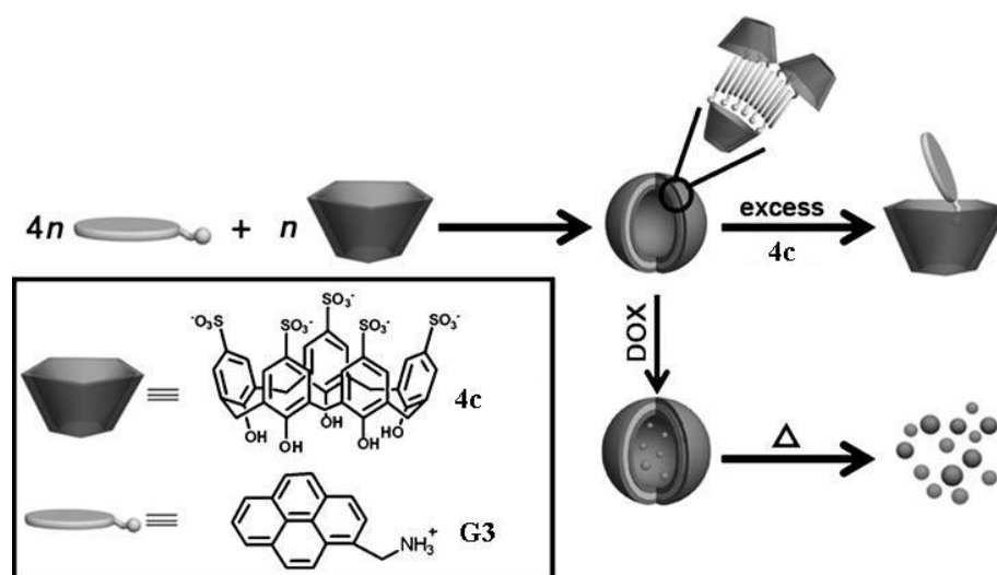
Figure 11. Formation of supramolecular binary vesicles made from pyrene derivative G3 and calixarene 4c (Reprinted with permission from ref. [75]. Copyright 2010 Wiley-VCH).
