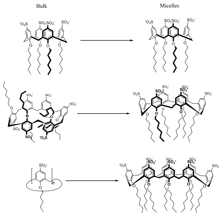
Figure 6. Conformational reorganization of amphiphilic p -sulfonatocalix[ n ]arenes upon micellization.
