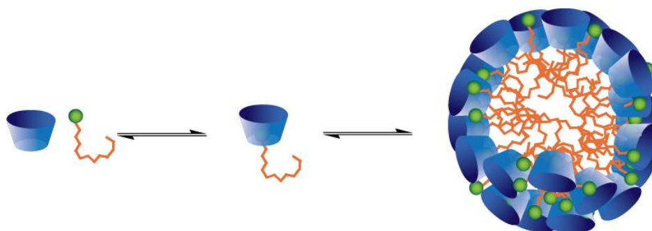
Figure 10. Promoted aggregation of alkyltrimethylammonium surfactants through the formation of host-guest complexes with calix[6]arene 4a (Reprinted with permission from ref. [66]. Copyright 2012, American Chemical Society).
