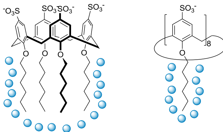
Figure 8. Conformation-dependent hydration of the alkyl chains of p -sulfonatocalix[ n ]arenes.
