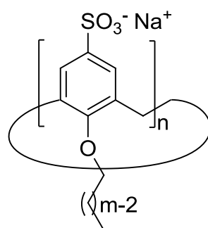
Figure 4. Amphiphilic p -sulfonatocalix[ n ]arenes used to establish structure aggregation relationships in references [60,61].
