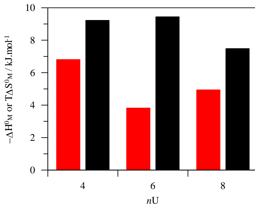
Figure 7. Variation of the enthalpy (red bars) and entropy (black bars) of micellization with the number of monomeric units ( nU ) present in the structure of the amphiphilic p -sulfonatocalix[ n ]arenes. All data is given in \text{kJ mol}^{-1} of alkyl chain units.
