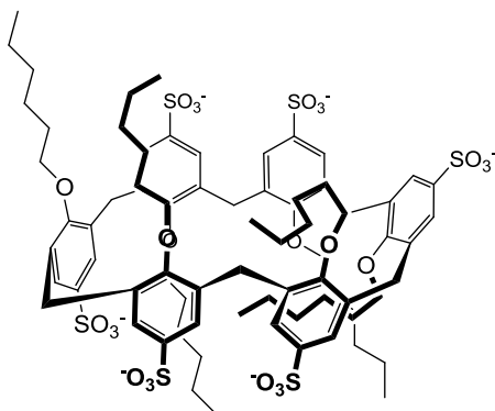
Figure 5. Pseudo 1,2,3-alternate conformation adopted by calix[6]arene 3d below the CMC.
