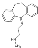
Nortriptyline
