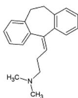
Amitriptyline
