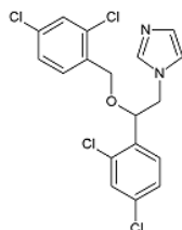
Miconazole
