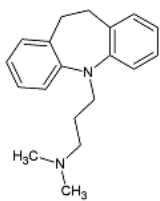
Imipramine
