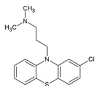
Chlorpromazine
