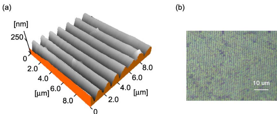
Figure 4. (a) AFM and (b) optical images of SRG inscribed on AAB single crystal.
