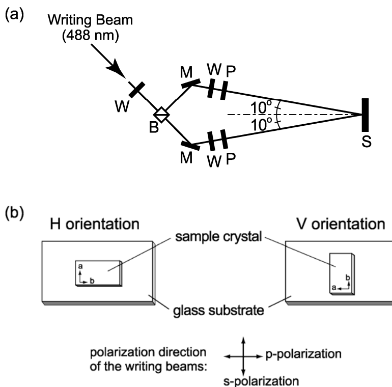
Figure 3. (a) Schematic experimental setup for photoinduced SRG formation. S: sample, P: polarizer, W: wave plate, M: mirror, B: beam splitter. (b) Schematic illustration of the sample orientation.
