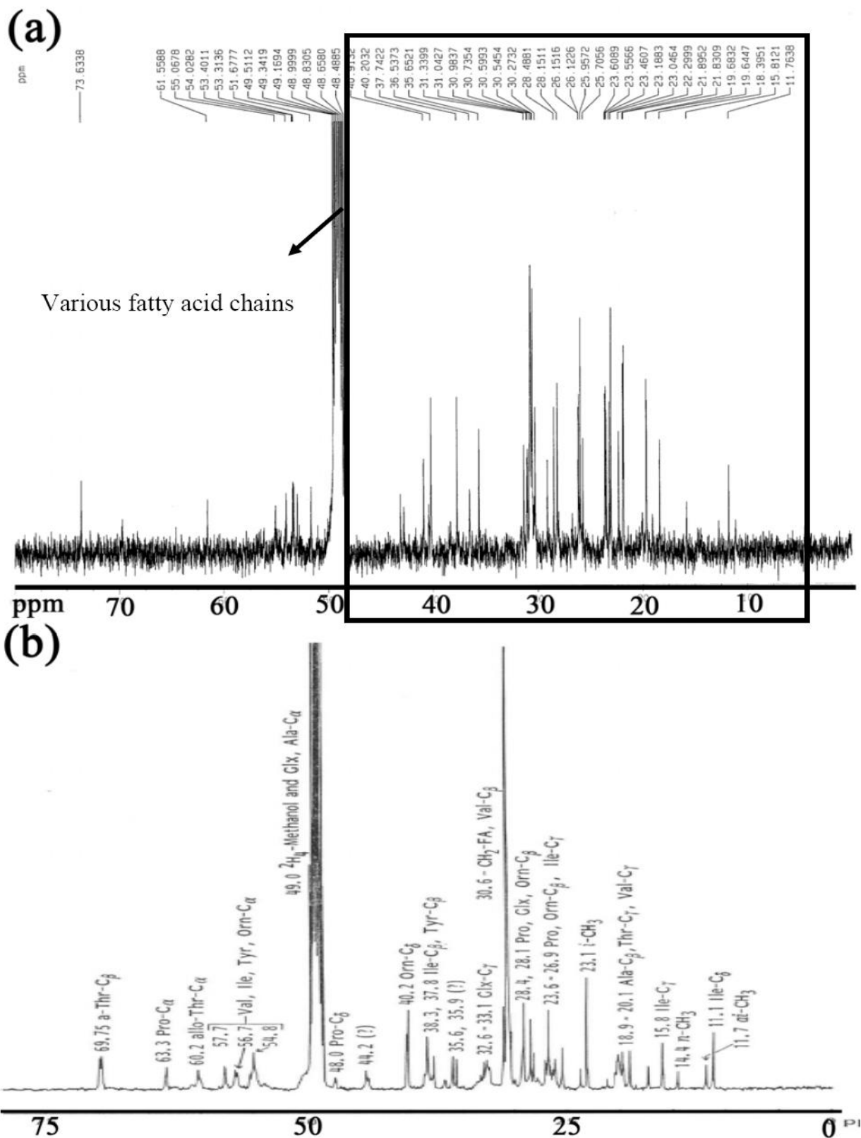
Figure S2. (a) ^{13}\text{C} -NMR spectrum for fengycin product obtained in this work; (b) ^{13}\text{C} -NMR spectrum of fengycin from literature [14]; (c) ^{13}\text{C} -NMR spectrum for fengycin product obtained in this work; (d) ^{13}\text{C} -NMR spectrum of fengycin from literature [14]
