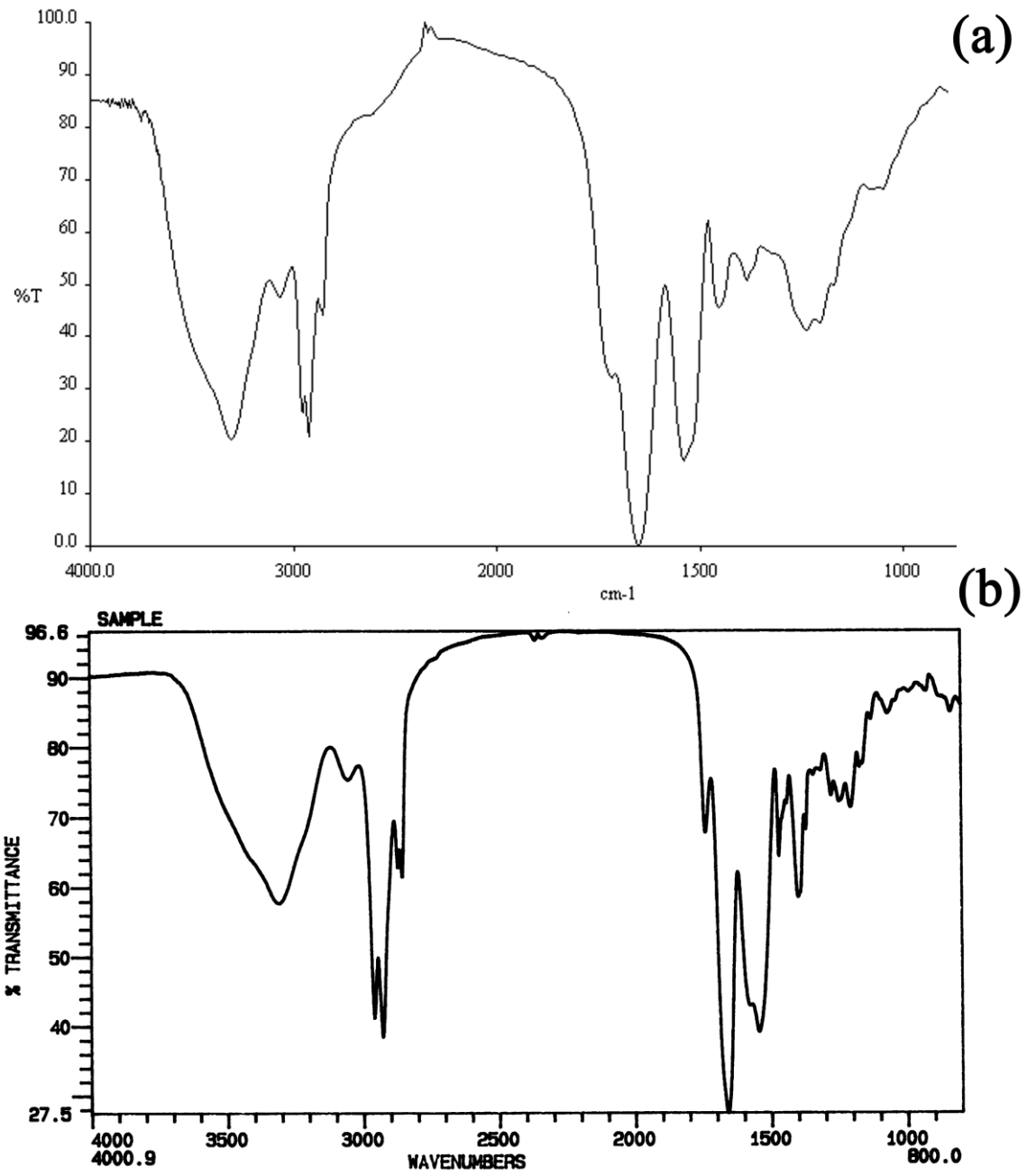
Figure S1. (a) Infrared spectrum for fengycin product obtained in this work; (b) Infrared spectrum of fengycin from literature [15].
