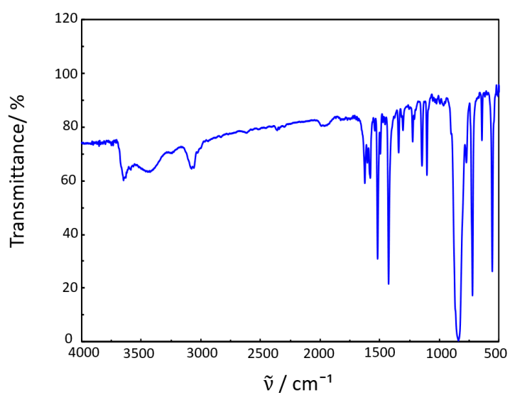
Figure S3. IR spectra of 3.
