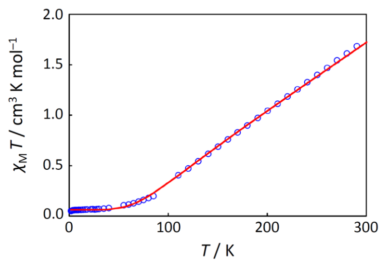
Figure S5. The \chi_M T versus T plot for 3 The observed data (○) and the theoretical curve (—).
