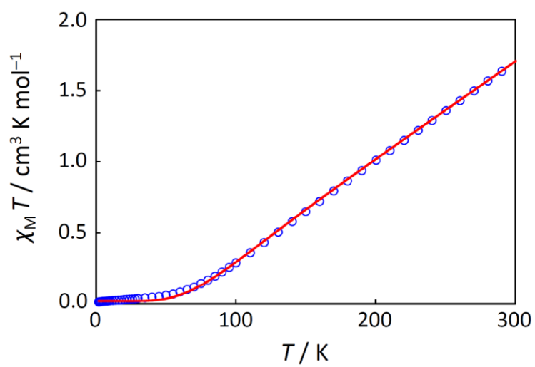
Figure S4. The \chi_M T versus T plot for 2. The observed data (○) and the theoretical curve (—).
