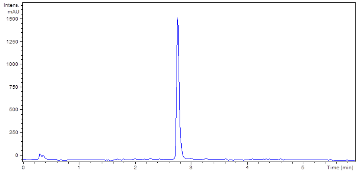
Compound 7b:
