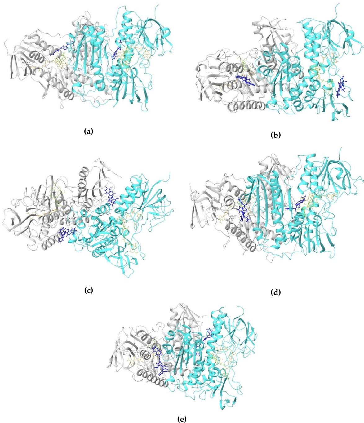
Figure S1. LmTR in complex with ZINC14970552 (a), ZINC09642432 (b), ZINC04684558 (c), ZINC11841871 (d) and ZINC12151998 (e). The LmTR monomers A and B are represented with gray ribbons and cyan ribbons, respectively. The ligands are represented in blue sticks FAD and NADH are represented in thin sticks yellow and green, respectively.
