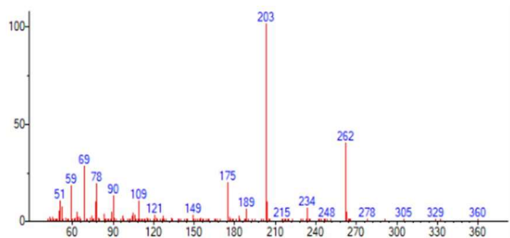
Unknown 20 (TFA derivative)
