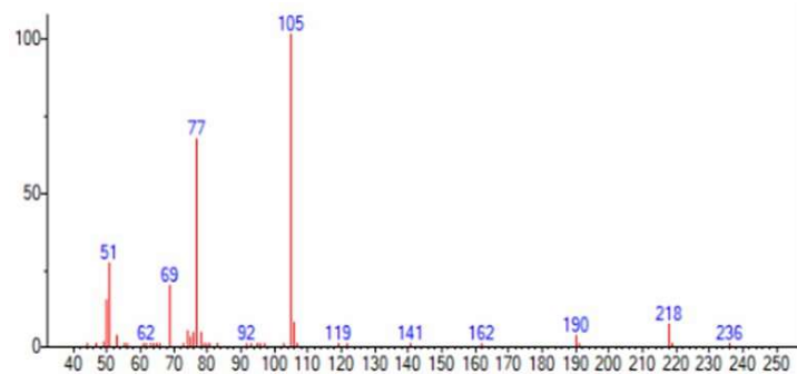
Unknown 17 (TFA derivative)
