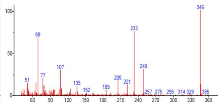
Vanillyl alcohol (TFA di-derivative)
