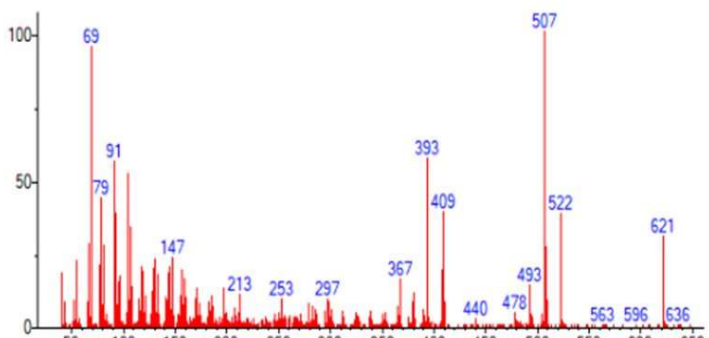
Unknown 22 (TFA derivative)
