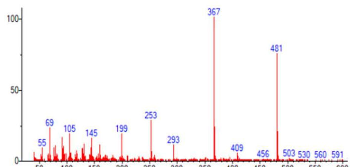
Unknown 21 (TFA derivative)
