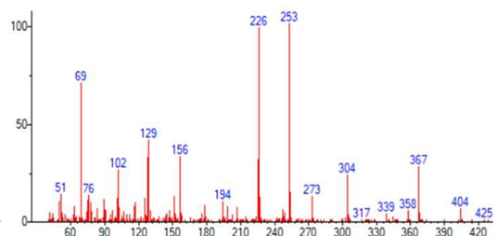
Unknown 19 (TFA derivative)
