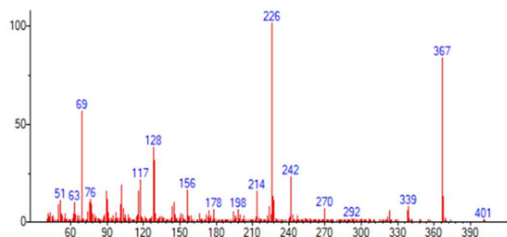
Unknown 18 (TFA derivative)
