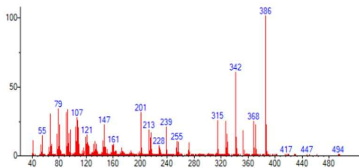
Epiandrosterone (TFA derivative)
