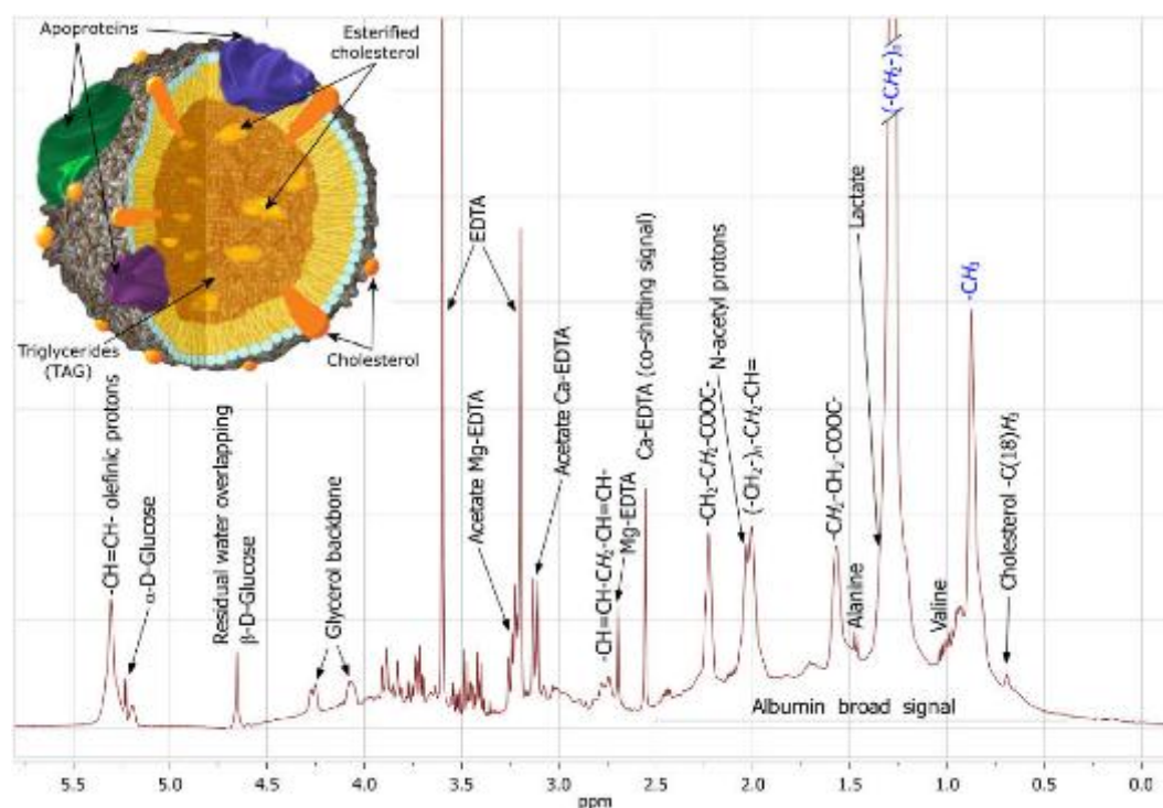
Figure 41. Representative ^1\text{H} -NMR spectrum (500 MHz) of human blood. Inset shows a schematic view of the micellar chylomicron structure. Adopted, with permission, from [202]. Copyright 2010, BioMed Central Ltd.
