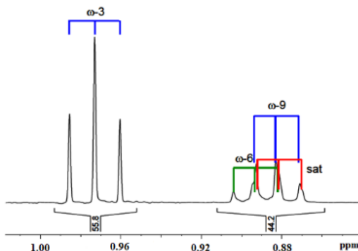
Figure 7. Separation of \omega -3 from \omega -6, \omega -9 and saturated fatty acids on the basis of 1 H-NMR chemical shifts of –CH 3 groups. Free download from: http://www.ilps.org/index.php/Standardized_Methods.html .
