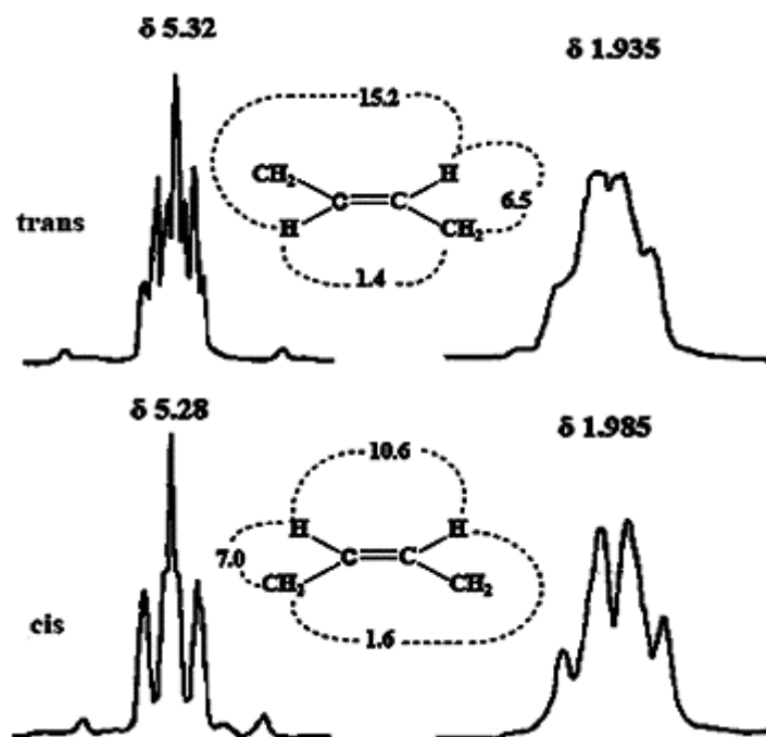
Figure 6. Computer simulated ^1\text{H} -NMR signals for alkenyl and allylic protons in isolated cis and trans double bonds. Adopted, with permission, from [54]. Copyright 1975, North-Holland Publishing Company.
