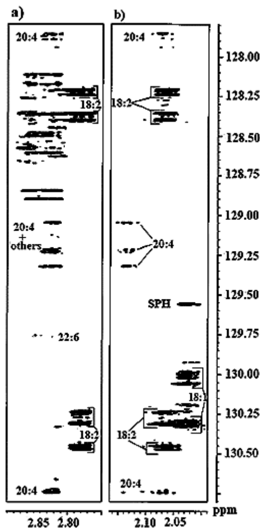
Figure 40. Semi-selective 800 MHz HSQC-TOCSY spectrum of the double bond region of blood plasma lipids. (a) Correlations to the allylic \Delta\text{-CH}_2\text{-}\Delta protons (ca. 2.8 ppm) (b); \Delta\text{-}^1\text{CH} protons (ca. 2.05 ppm). In the \Delta\text{-CH}_2\text{-}\Delta region the 18:2 signals are well separated from the higher polyunsaturated fatty acids, whereas in the \Delta\text{-}^1 region the 18:1 signals are separated from all other signals. The 20:4 fatty acid shows additional well separated signals at 2.13 ppm. Adopted, with permission, from [89]. Copyright 1998, John Wiley & Sons, Ltd.
