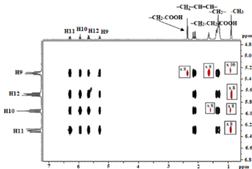
Figure 16. 500 MHz 1D ^1\text{H} -NMR spectrum of (9- cis , 11- trans ) 18:2 CLA in \text{CDCl}_3 (concentration: 10 mM, T: 298 K, acquisition time: 2.7 s, relaxation delay: 8 s, number of scans: 128, experimental time: ~23 min).
