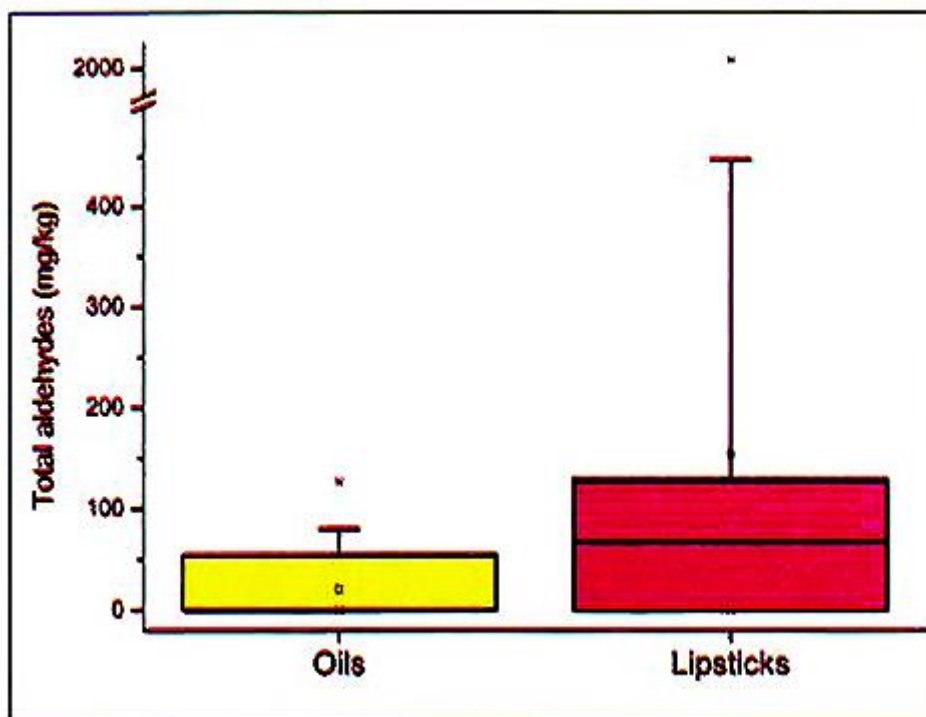
Figure 34. Total aldehydes in 72 oils and 38 cosmetics. The boxplot shows a statistical distribution (whiskers: minimum and maximum (max 1.5 times the length of the inner quartiles; data points outside are outliers). Adopted, with permission, from [168]. Copyright 2010, John Wiley & Sons Ltd.
