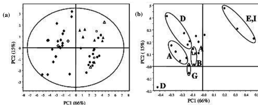
Figure 37. PCA of the ^1\text{H} -NMR resonances of lipid fractions: (a) score plot of PC1 vs. PC2 [training set ( \blacklozenge ) alpine farms; ( \bullet ) lowland industrialized factories, ( \blacktriangle ) mountain industrialized factories; test set ( \lozenge ) alpine farms; ( \circ ) lowland industrialized factories, ( \triangle ) mountain industrialized factories]; (b) loadings profile (letters correspond to Figure 36). Adopted, with permission, from [189]. Copyright 2008, American Chemical Society.
