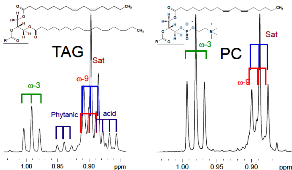
Figure 24. ^1\text{H} -NMR spectra of TAG and phospholipids from krill oil after preparative separation. The neutral lipids fraction contains the branched phytanic acid which can also be quantified. Free download from: http://www.ilps.org/index.php/Standardized_Methods.html .
