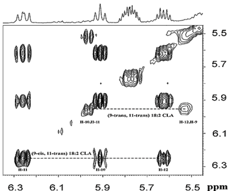
Figure 26. 500MHz ^1\text{H} - ^1\text{H} TOCSY NMR spectrum of the lipid fraction of a lyophilized milk sample in \text{CDCl}_3 with suppression of two major lipid proton resonances at 1.27 and 5.35 ppm. Experimental conditions: 298 K, 32 repetitions of 256 increments, total experimental time 5 h 5 min. Adopted, with permission, from [56]. Copyright 2014, Elsevier B.V.
