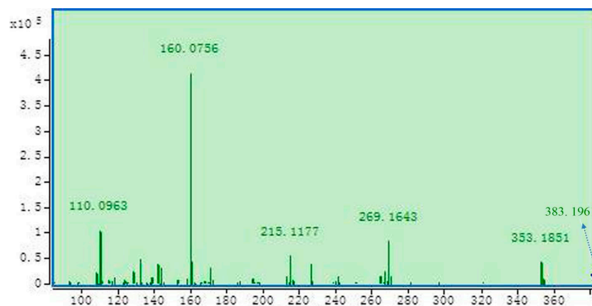
Figure S3. The MS spectra of the possible intermediate.
