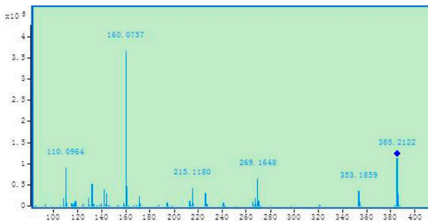
Figure S1. The MS spectra of rhynchophylline.
