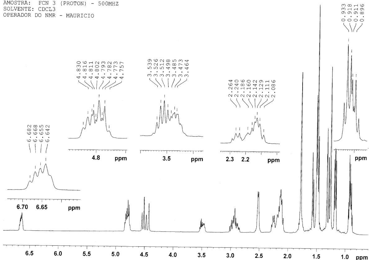
Figure S1. ^1\text{H} -NMR spectrum of compound 1 at 500 MHz in \text{CDCl}_3 .
