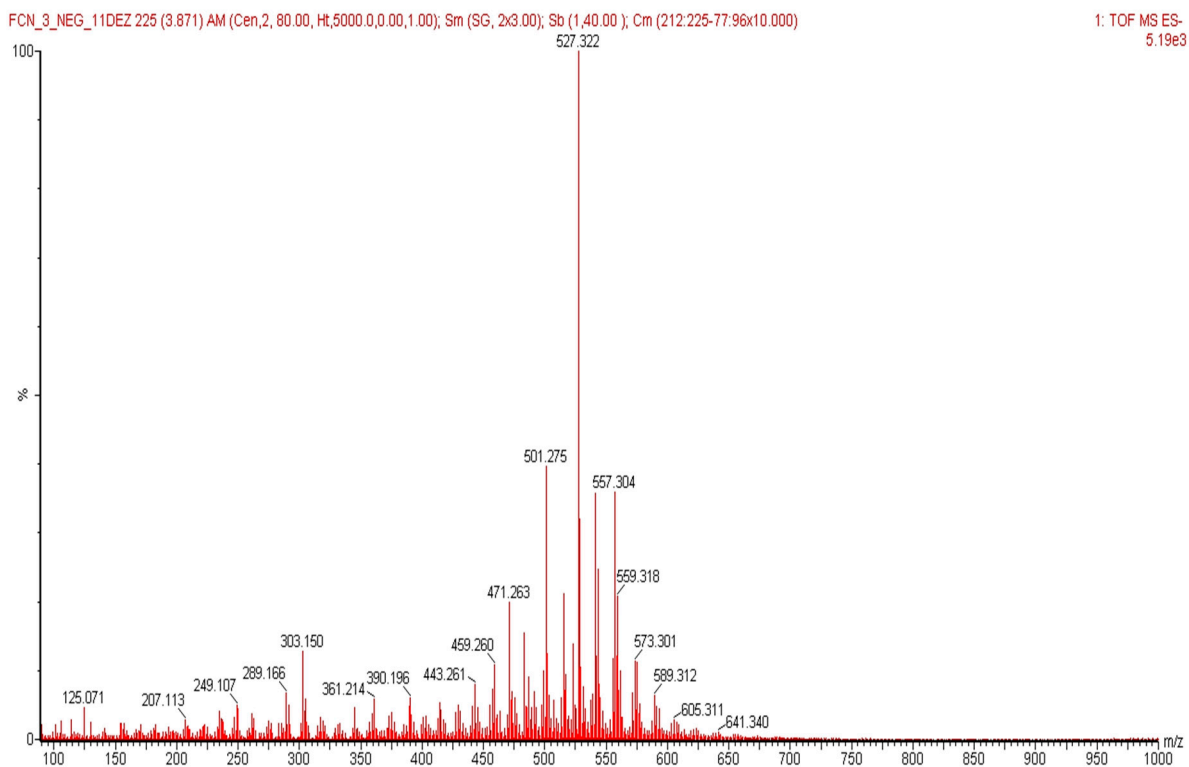
Figure S2. TOF-ESI-MS spectrum of compound 1 .
