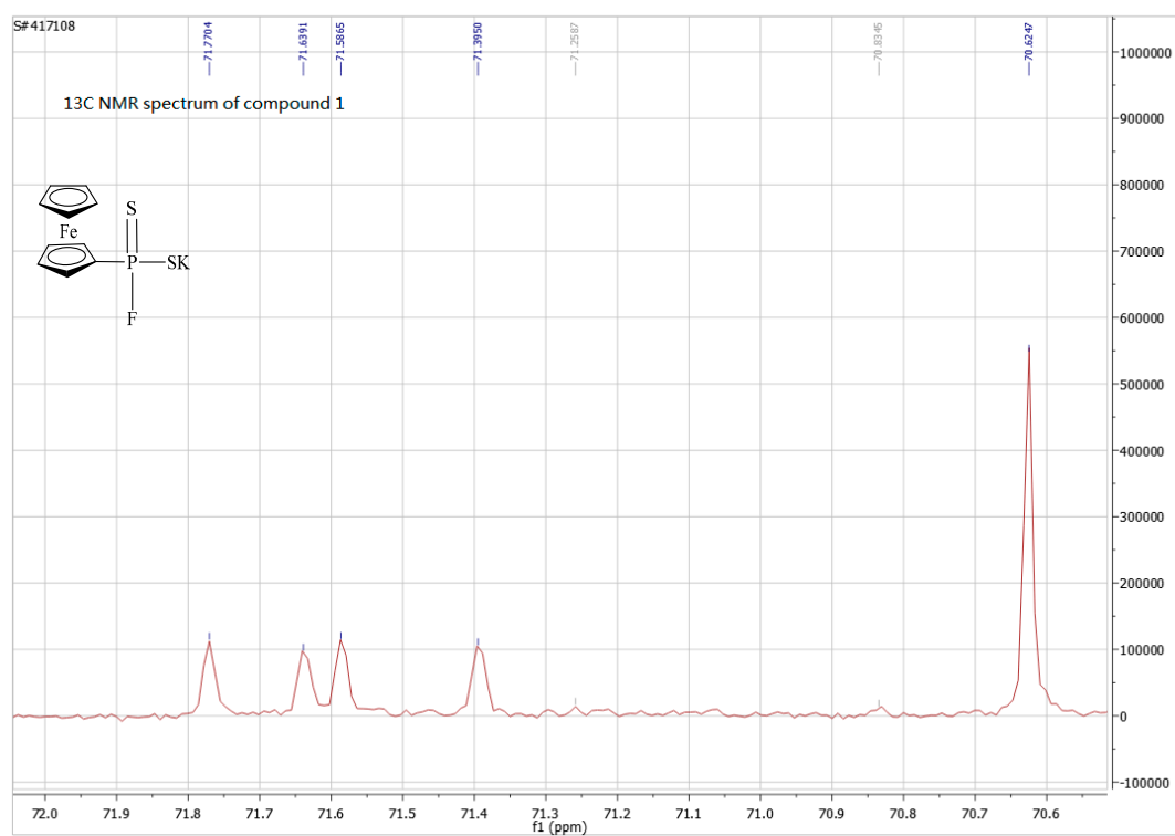
Figure S2. 13 C-NMR spectra of compound 1.
