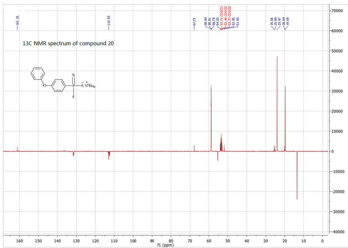
Figure S34. 13 C-NMR spectra of compound 20.
