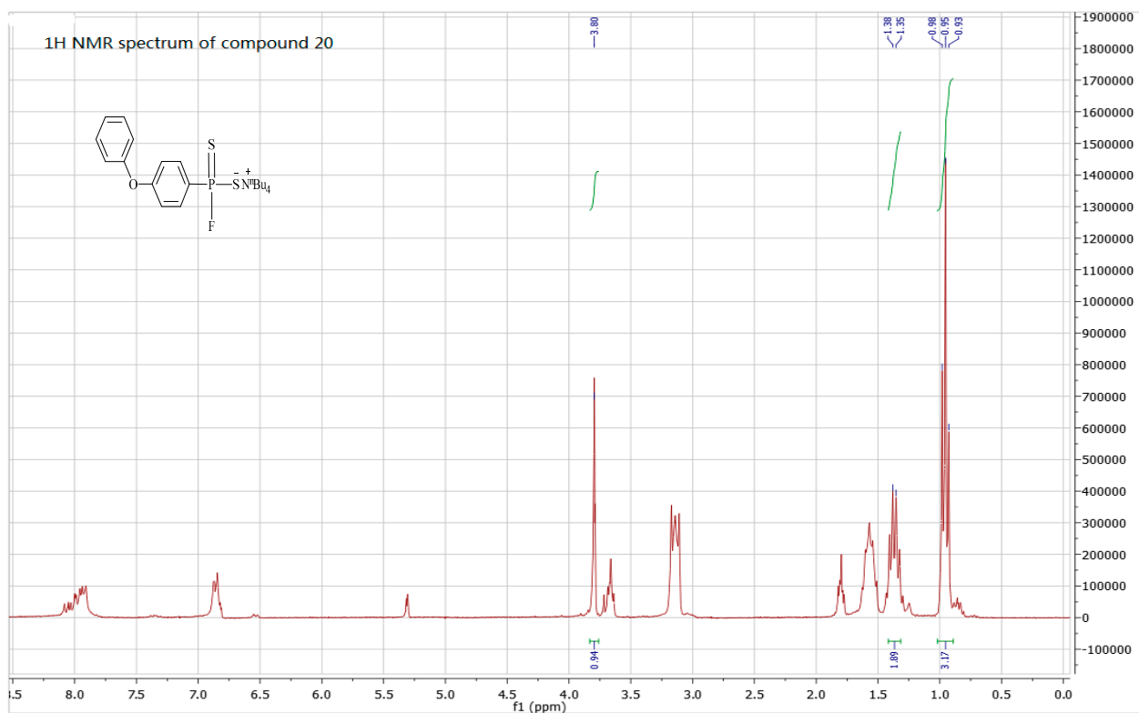
Figure S33. 1 H-NMR spectra of compound 20.
