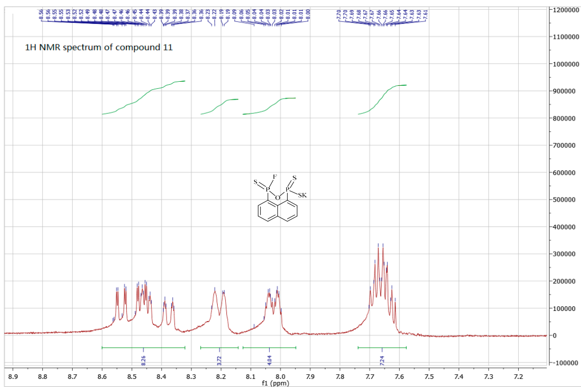
Figure S19. ^1\text{H} -NMR spectra of compound 11 .
