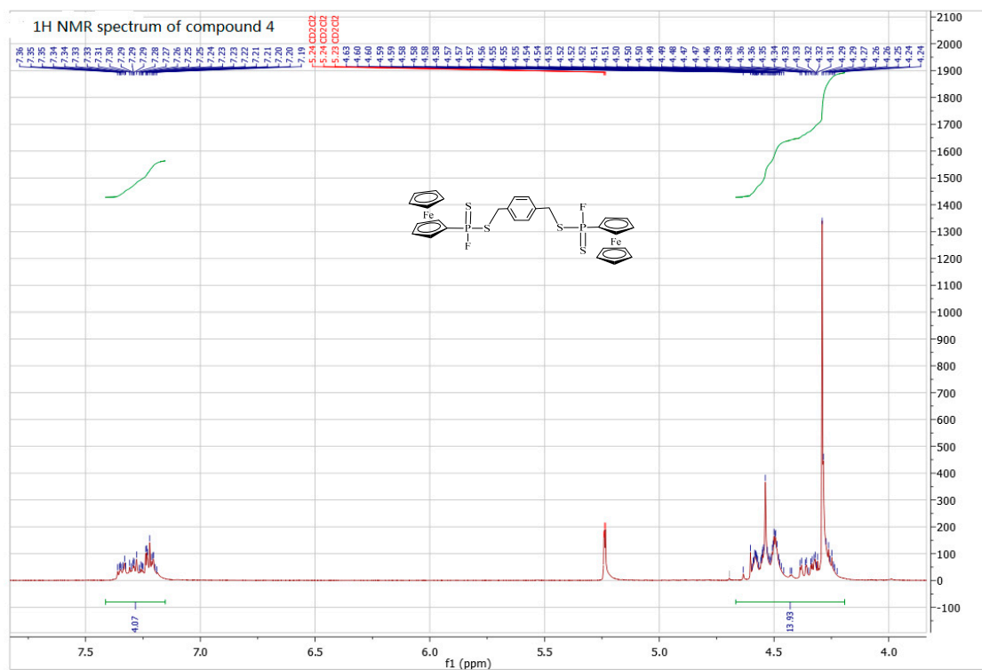
Figure S7. 1 H-NMR spectra of compound 4.
