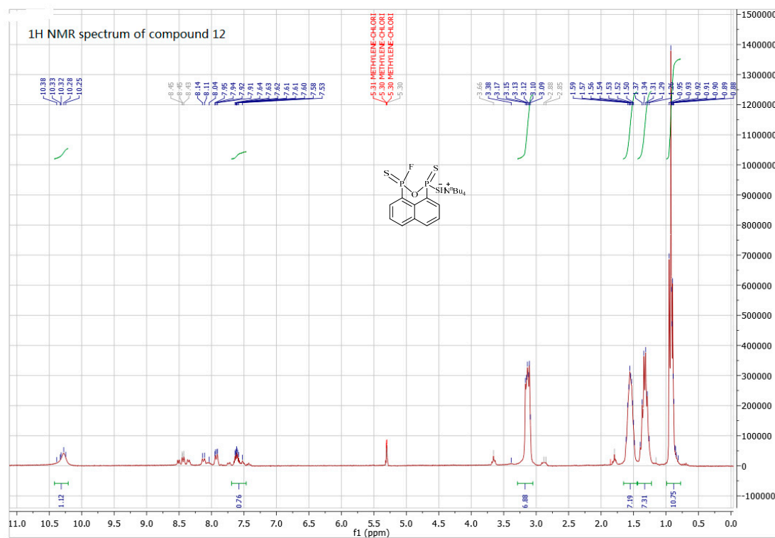
Figure S21. 1 H-NMR spectra of compound 12.
