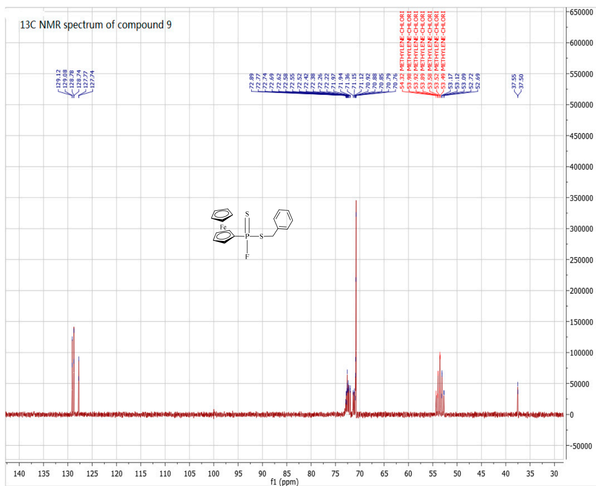
Figure S18. 13 C-NMR spectra of compound 9.
