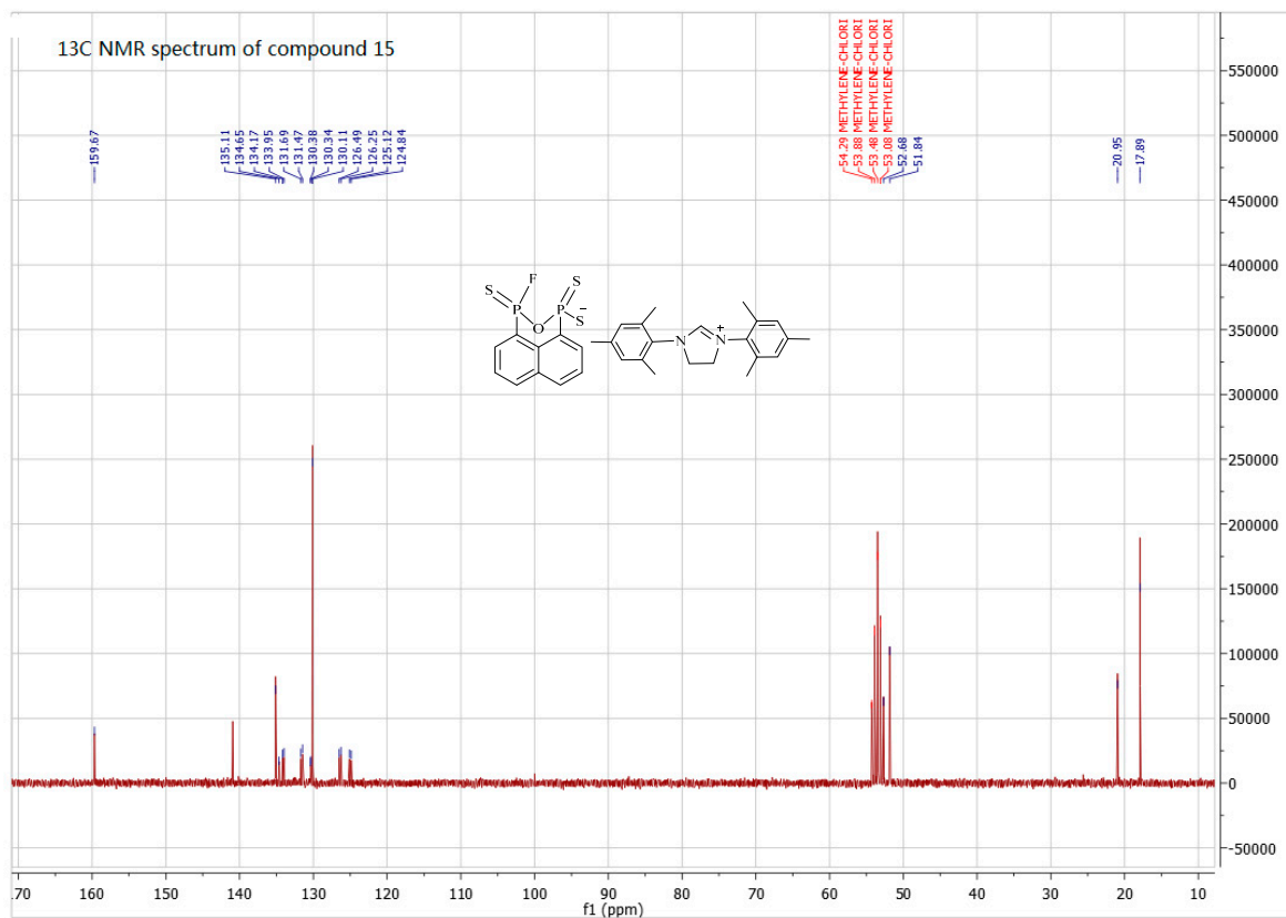
Figure S28. 13 C-NMR spectra of compound 15.
