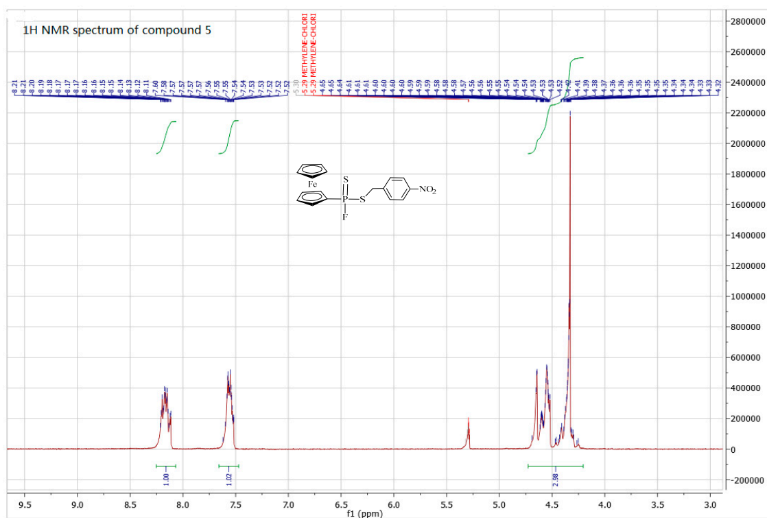
Figure S9. 1 H-NMR spectra of compound 5.
