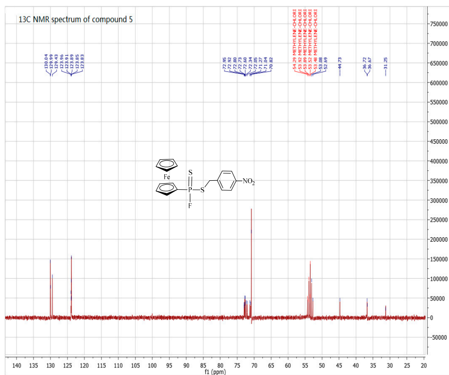
Figure S10. 13 C-NMR spectra of compound 5.
