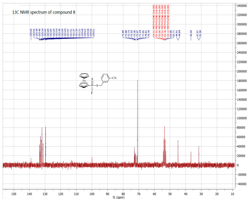
Figure S16. 13 C-NMR spectra of compound 8.
