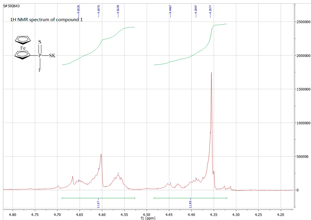
Figure S1. 1 H-NMR spectra of compound 1.
