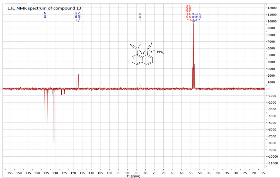
Figure S24. ^{13}\text{C} -NMR spectra of compound 13 .
