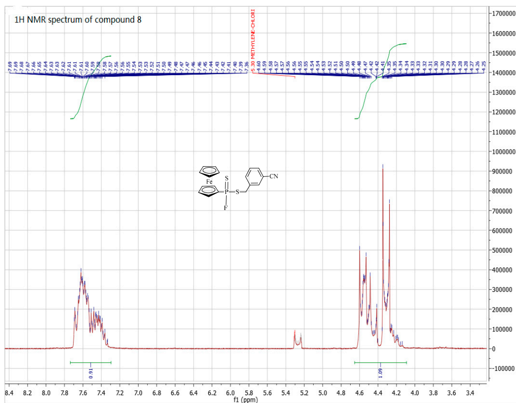
Figure S15. 1 H-NMR spectra of compound 8.
