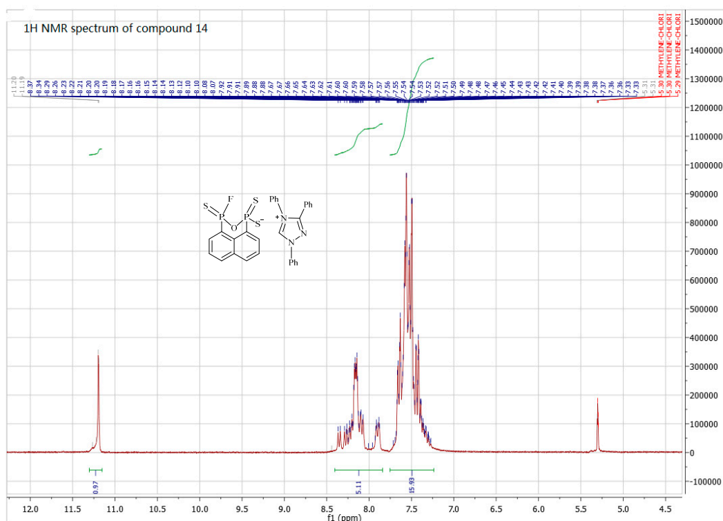
Figure S25. ^1\text{H} -NMR spectra of compound 14.
