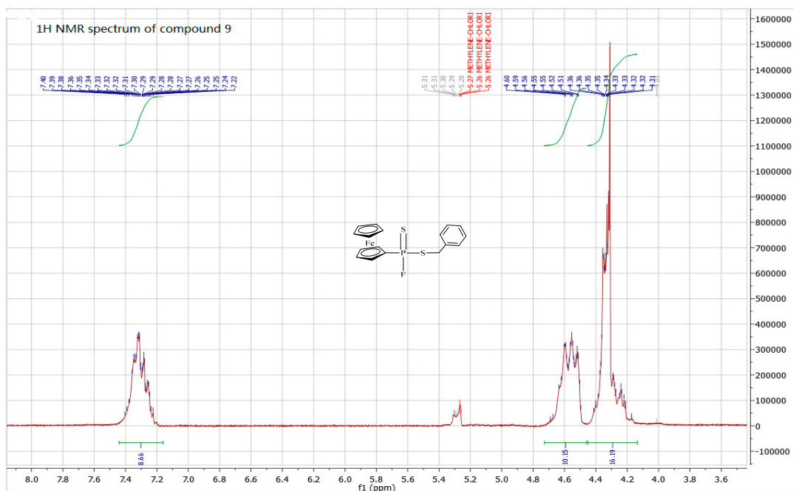
Figure S17. 1 H-NMR spectra of compound 9.
