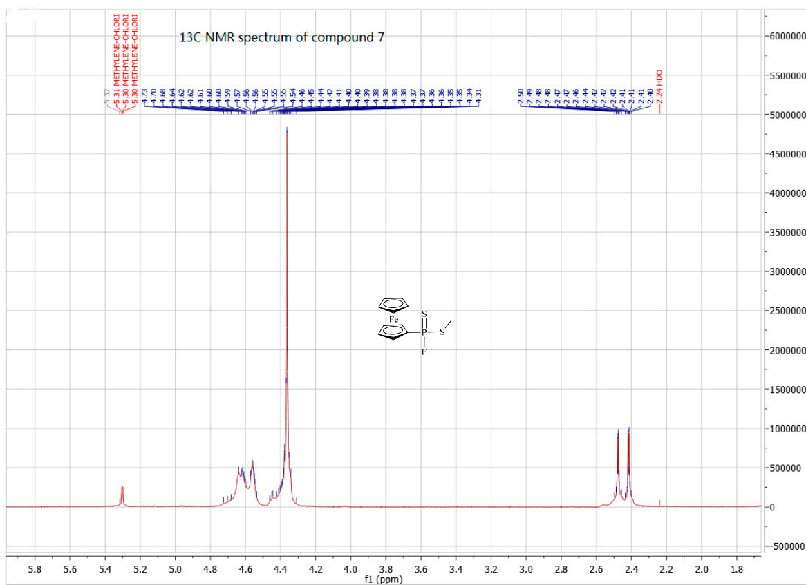
Figure S14. 13 C-NMR spectra of compound 7.
