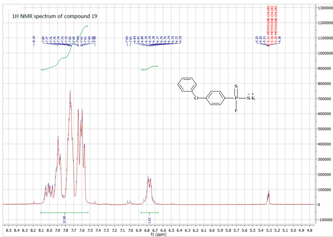
Figure S31. 1 H-NMR spectra of compound 19.
