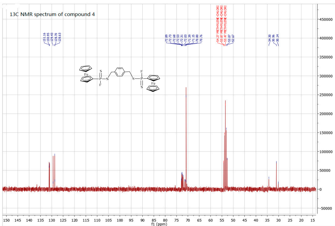
Figure S8. 13 C-NMR spectra of compound 4.
