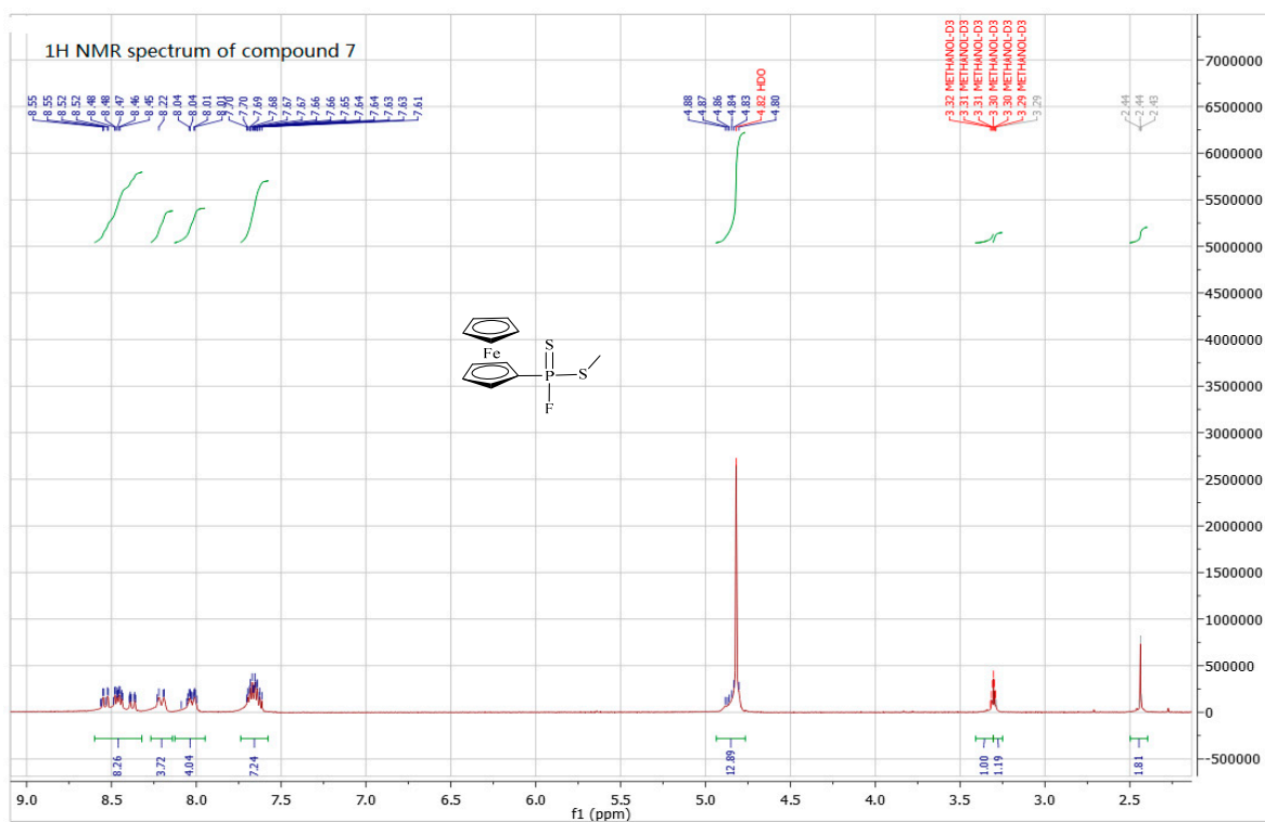
Figure S13. 1 H-NMR spectra of compound 7.
