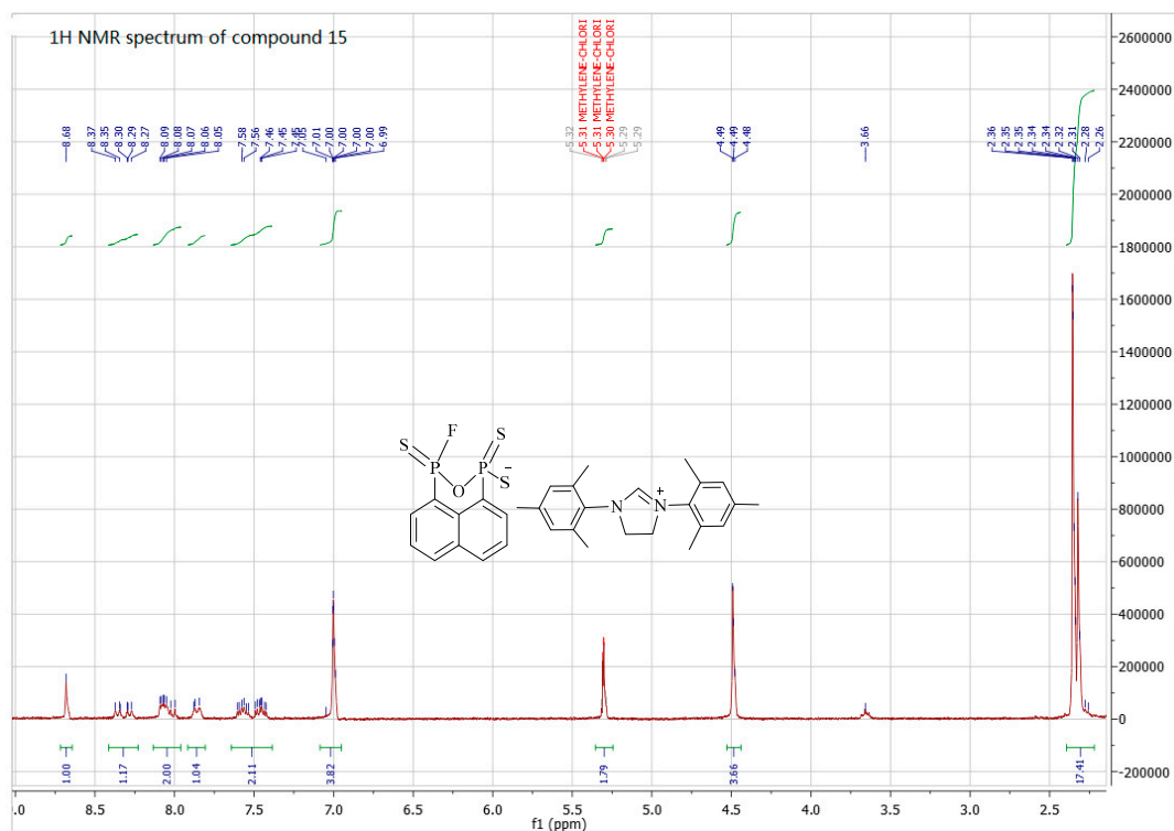
Figure S27. 1 H-NMR spectra of compound 15.
