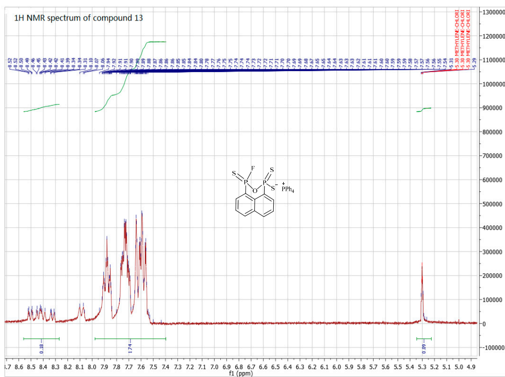
Figure S23. ^1\text{H} -NMR spectra of compound 13 .
