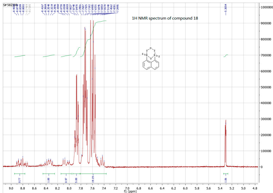
Figure S29. 1 H-NMR spectra of compound 18.
