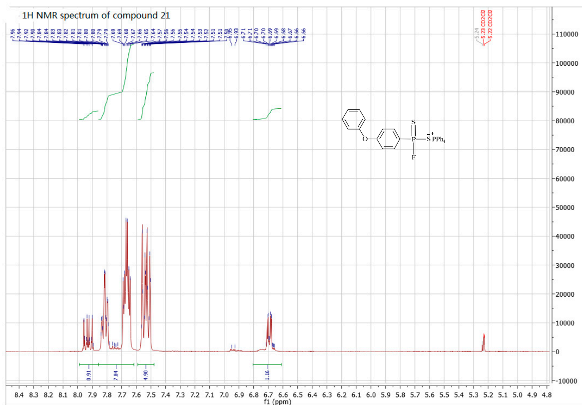
Figure S35. 1 H-NMR spectra of compound 21.
