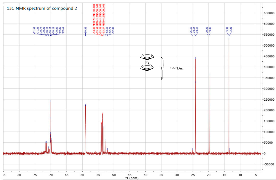
Figure S4. 13 C-NMR spectra of compound 2.
