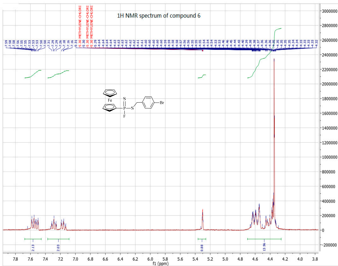
Figure S11. 1 H-NMR spectra of compound 6.
