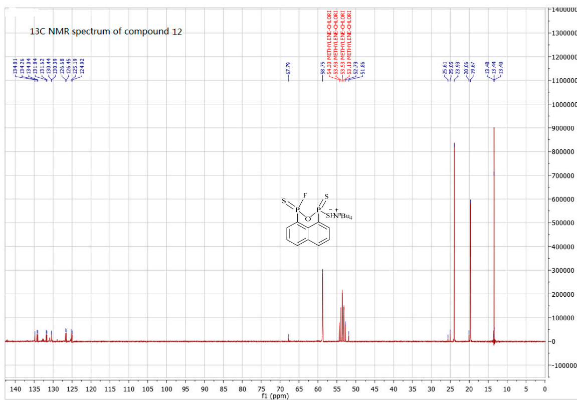
Figure S22. 13 C-NMR spectra of compound 12.
