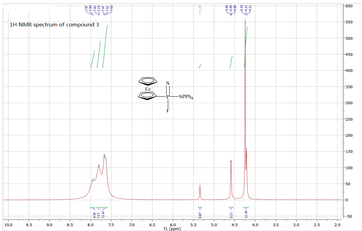
Figure S5. 1 H-NMR spectra of compound 3.
