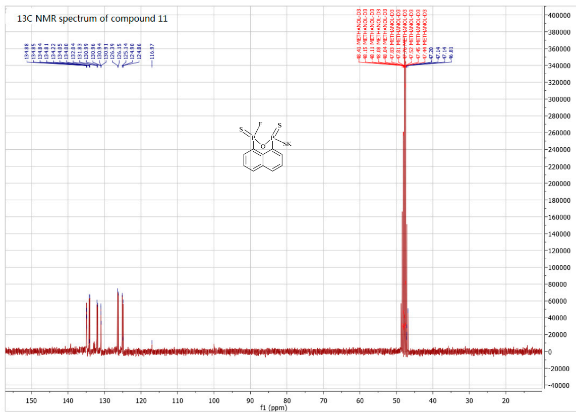
Figure S20. ^{13}\text{C} -NMR spectra of compound 11 .
