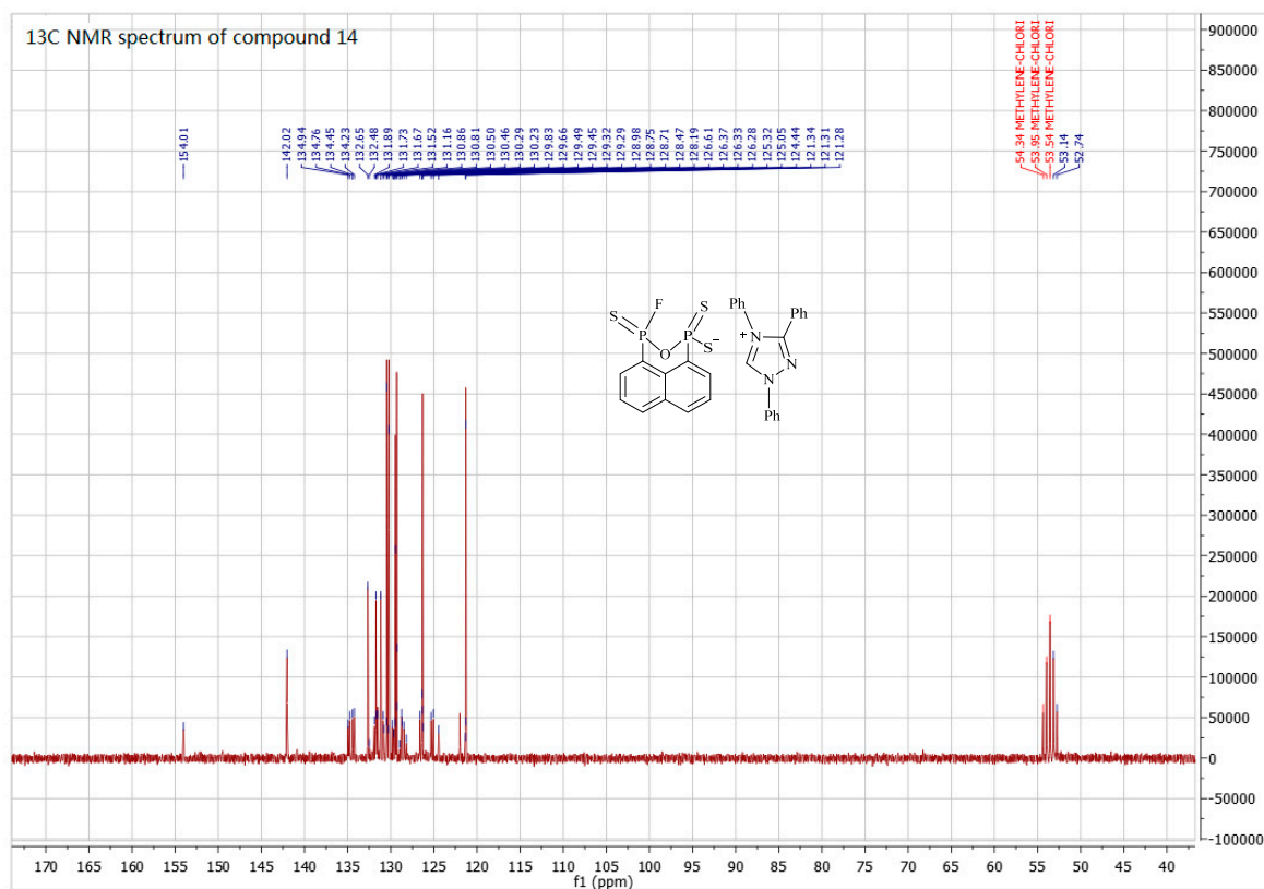
Figure S26. ^{13}\text{C} -NMR spectra of compound 14.
