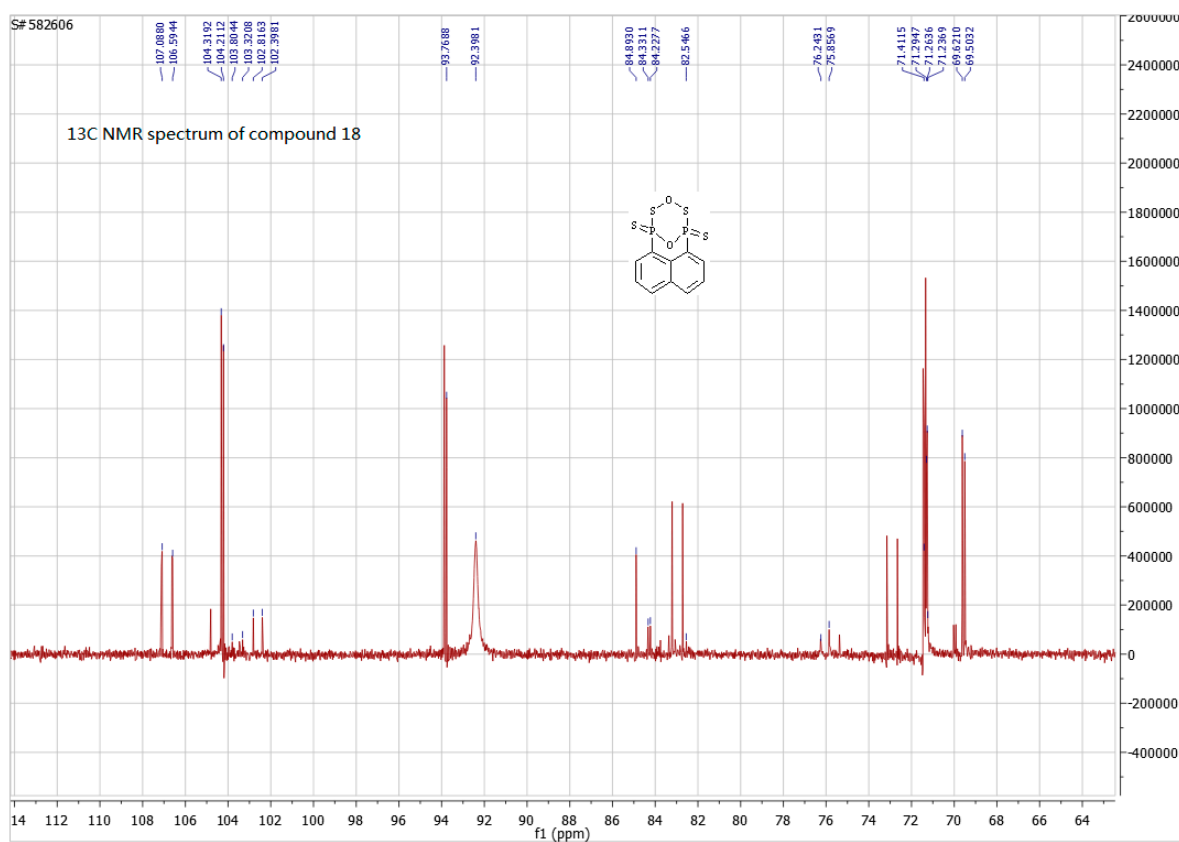
Figure S30. 13 C-NMR spectra of compound 18.
