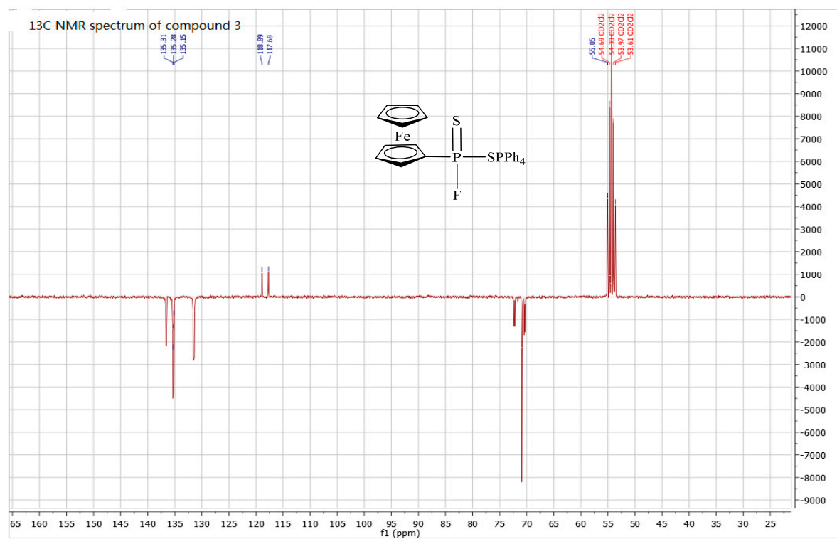
Figure S6. 13 C-NMR spectra of compound 3.
