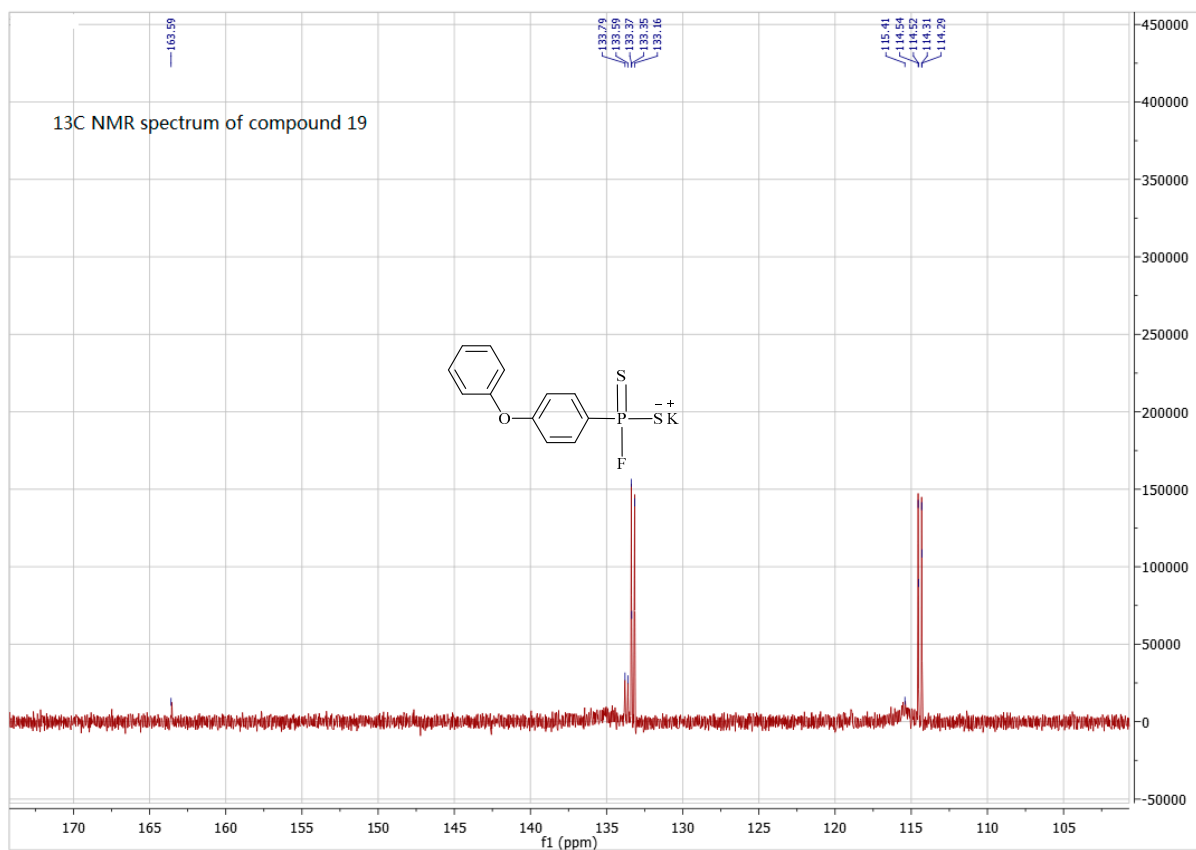
Figure S32. 13 C-NMR spectra of compound 19.
