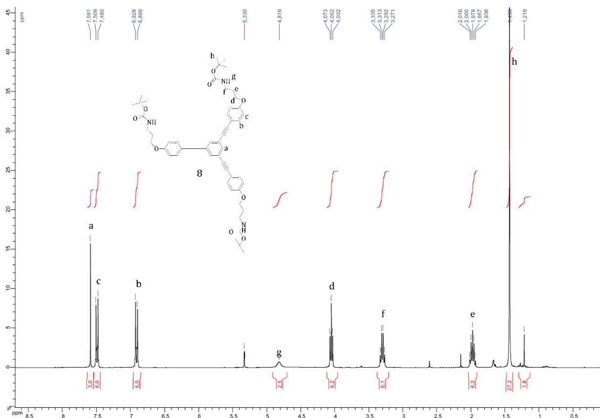
Figure S7. ^1\text{H} -NMR of compound 8 .
