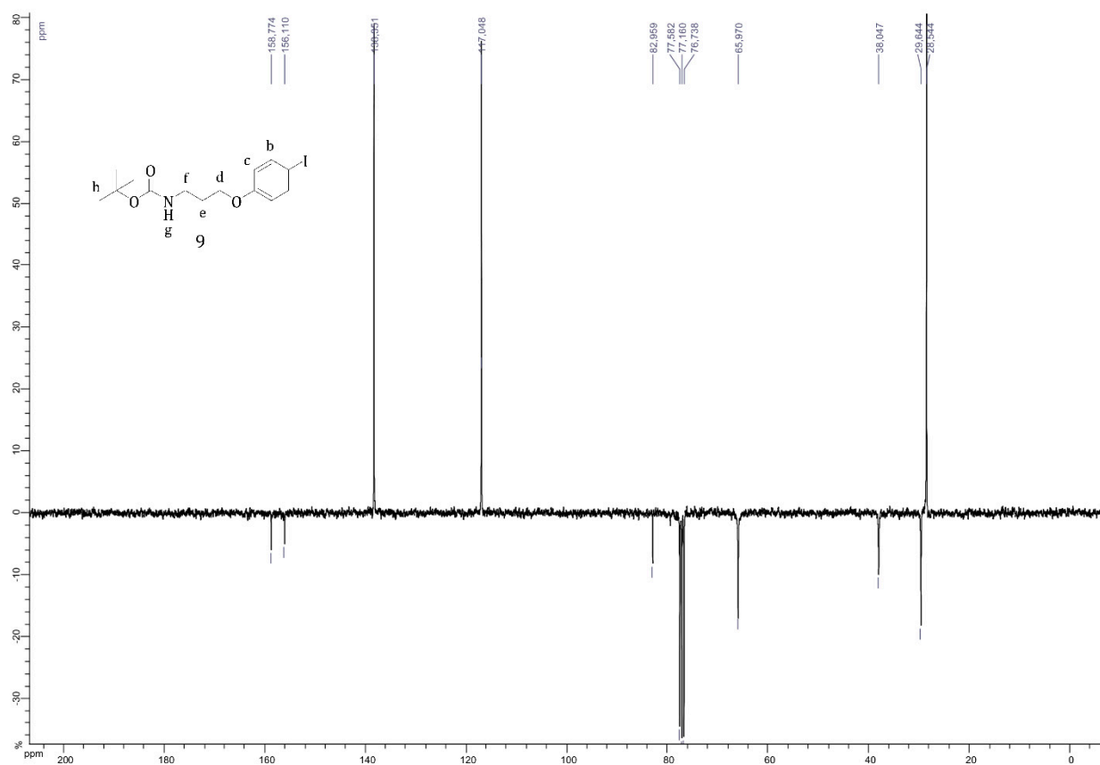
Figure S10. ^{13}\text{C} -NMR of compound 9 .
