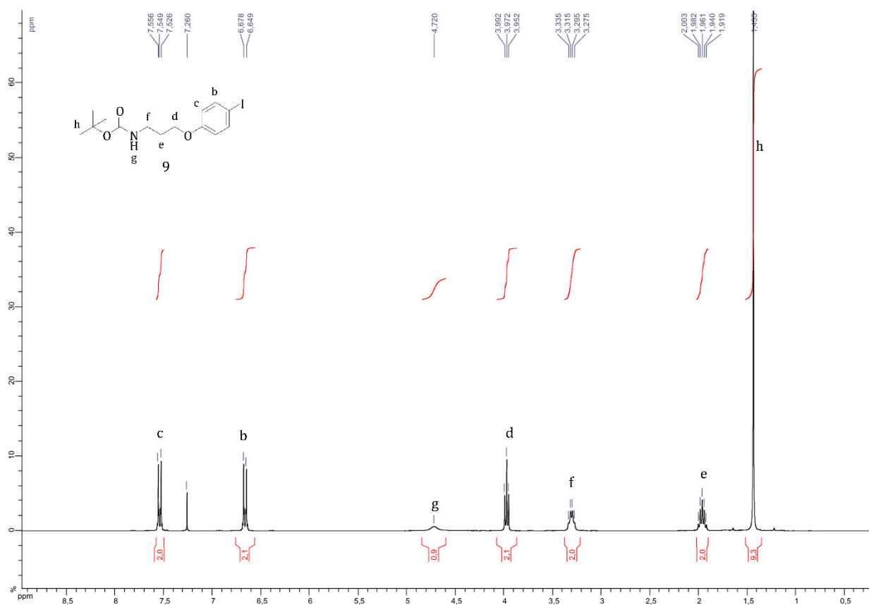
Figure S9. ^1\text{H} -NMR of compound 9 .
