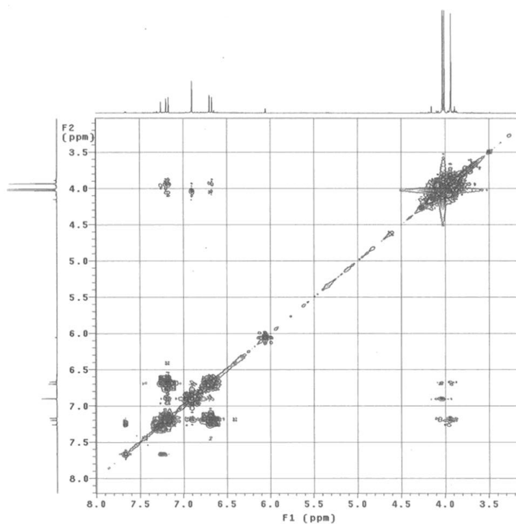
Figure S4. COSY spectrum of compound 1 .
