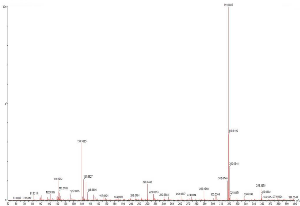
Figure S8. HRESIMS spectrum of compound 1 .
