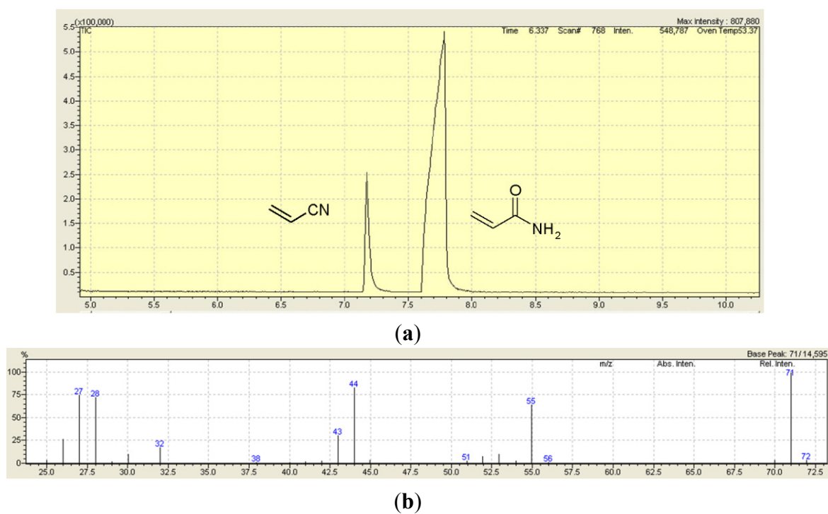
Figure S10. Acrylamide (Table 4, entry 9). (a) Retention time-intensity graph; and (b) m/z value-intensity graph.
