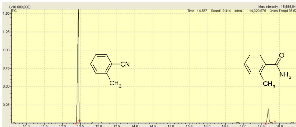
Figure S8. 2-methylbenzamide (Table 4, entry 7). (a) Retention time-intensity graph; and (b) m/z value-intensity graph.
