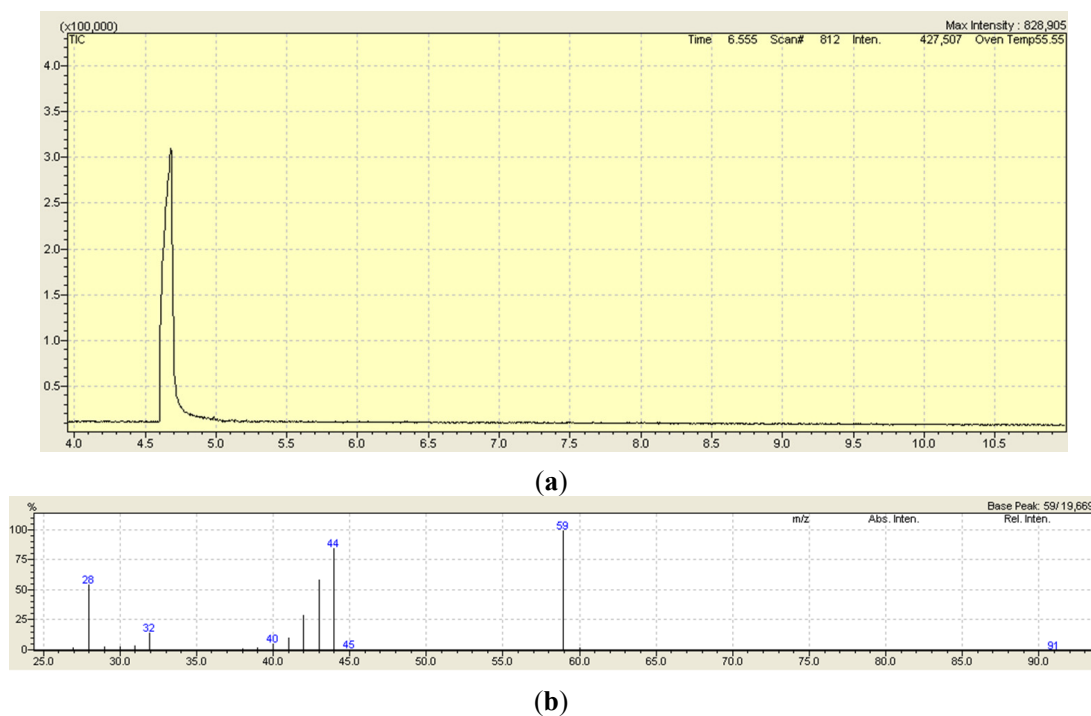
Figure S10. Acrylamide (Table 4, entry 9). (a) Retention time-intensity graph; and (b) m/z value-intensity graph.
