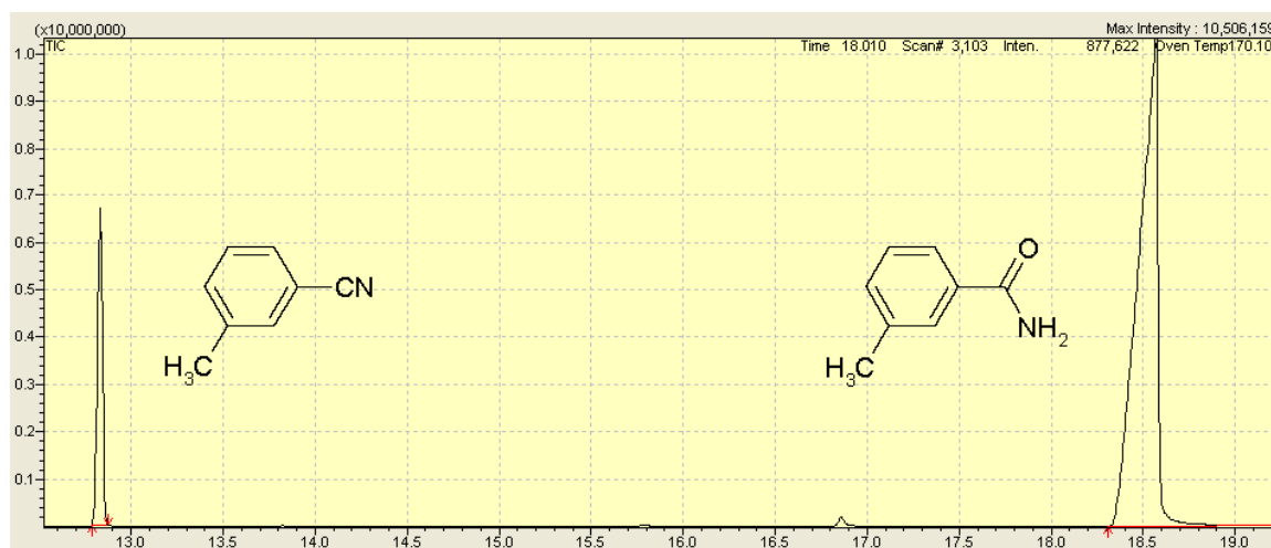
Figure S7. 3-methylbenzamide (Table 4, entry 6). (a) Retention time-intensity graph; and (b) m/z value-intensity graph.
