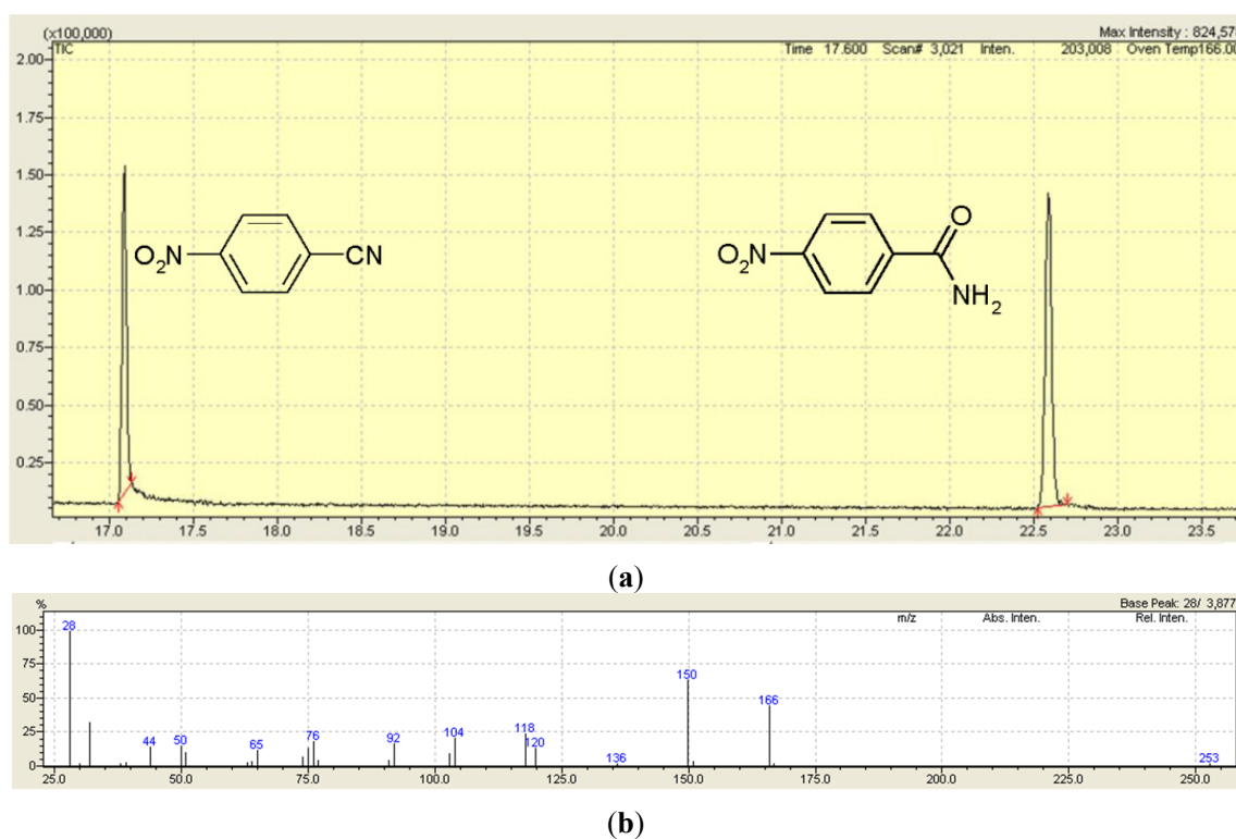
Figure S4. 4-nitrobenzamide (Table 4, entry 3). (a) Retention time-intensity graph; and (b) m/z value-intensity graph.
