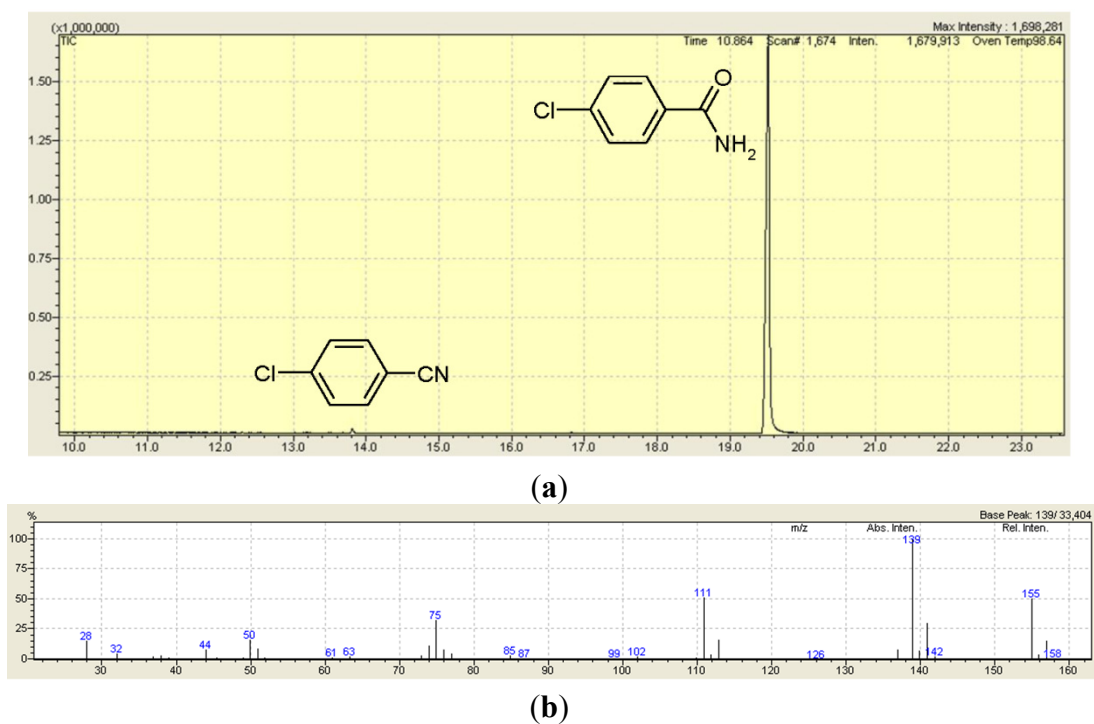
Figure S2. 4-Chlorobenzamide (Table 4, entry 1). (a) Retention time-intensity graph; and (b) m/z value-intensity graph.
