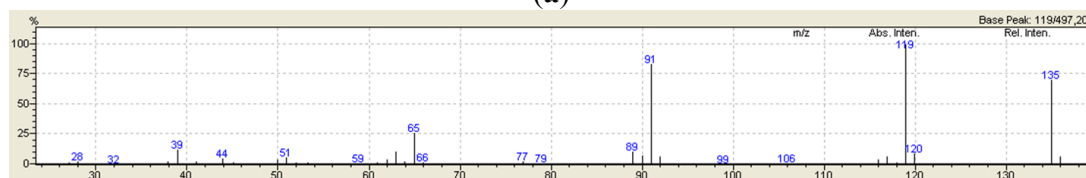
Figure S8. 2-methylbenzamide (Table 4, entry 7). (a) Retention time-intensity graph; and (b) m/z value-intensity graph.
