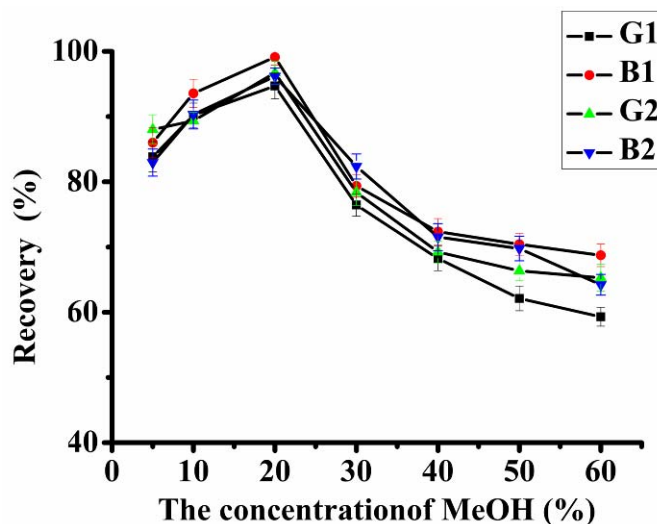
Figure 2. Effect of different loading solvents on the efficiency of IAC (aflatoxins spiked in peanut, 5 \mu\text{g}\cdot\text{kg}^{-1} each).
