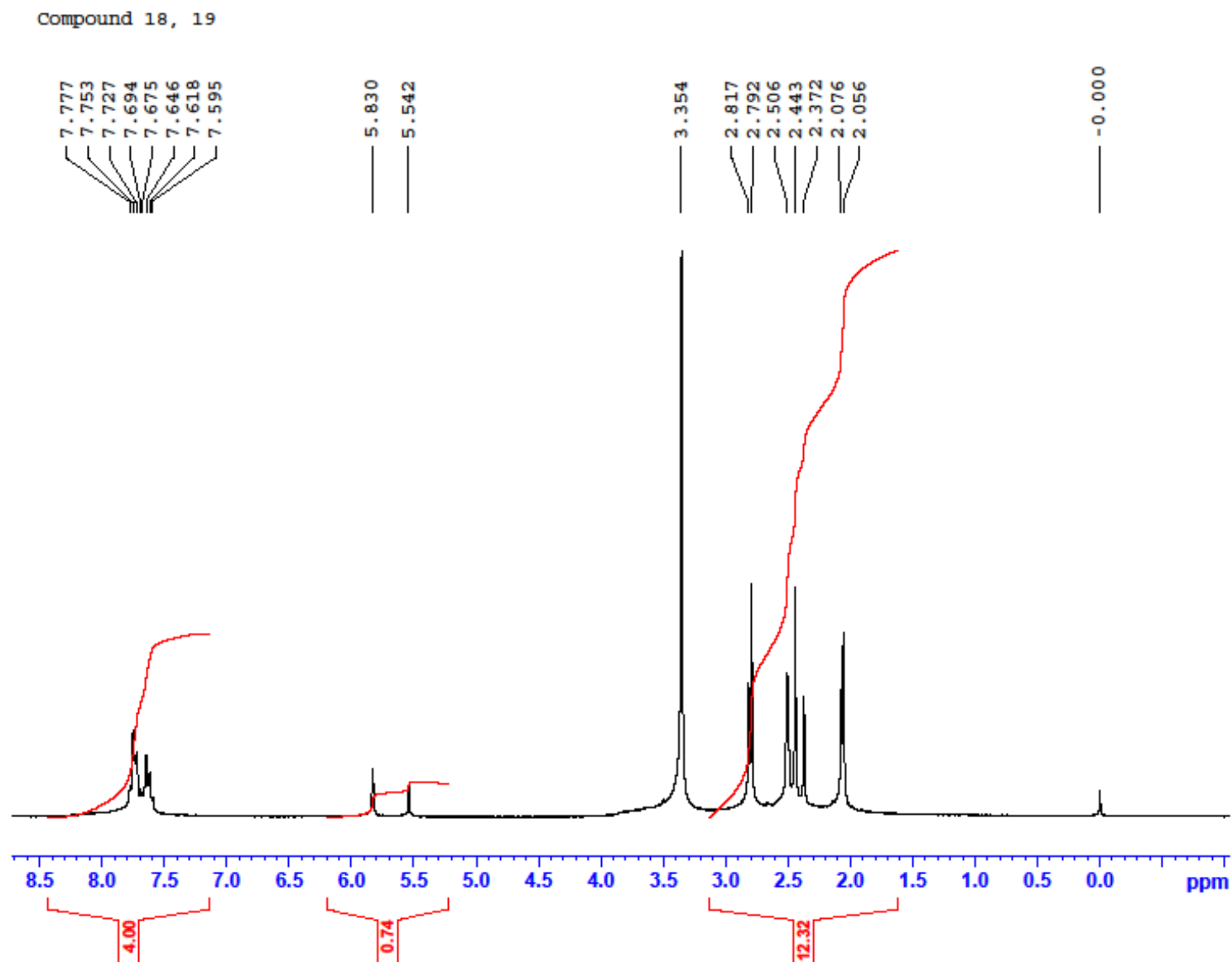
Figure S2. ^1\text{H-NMR} spectrum of compounds 18, 19.
