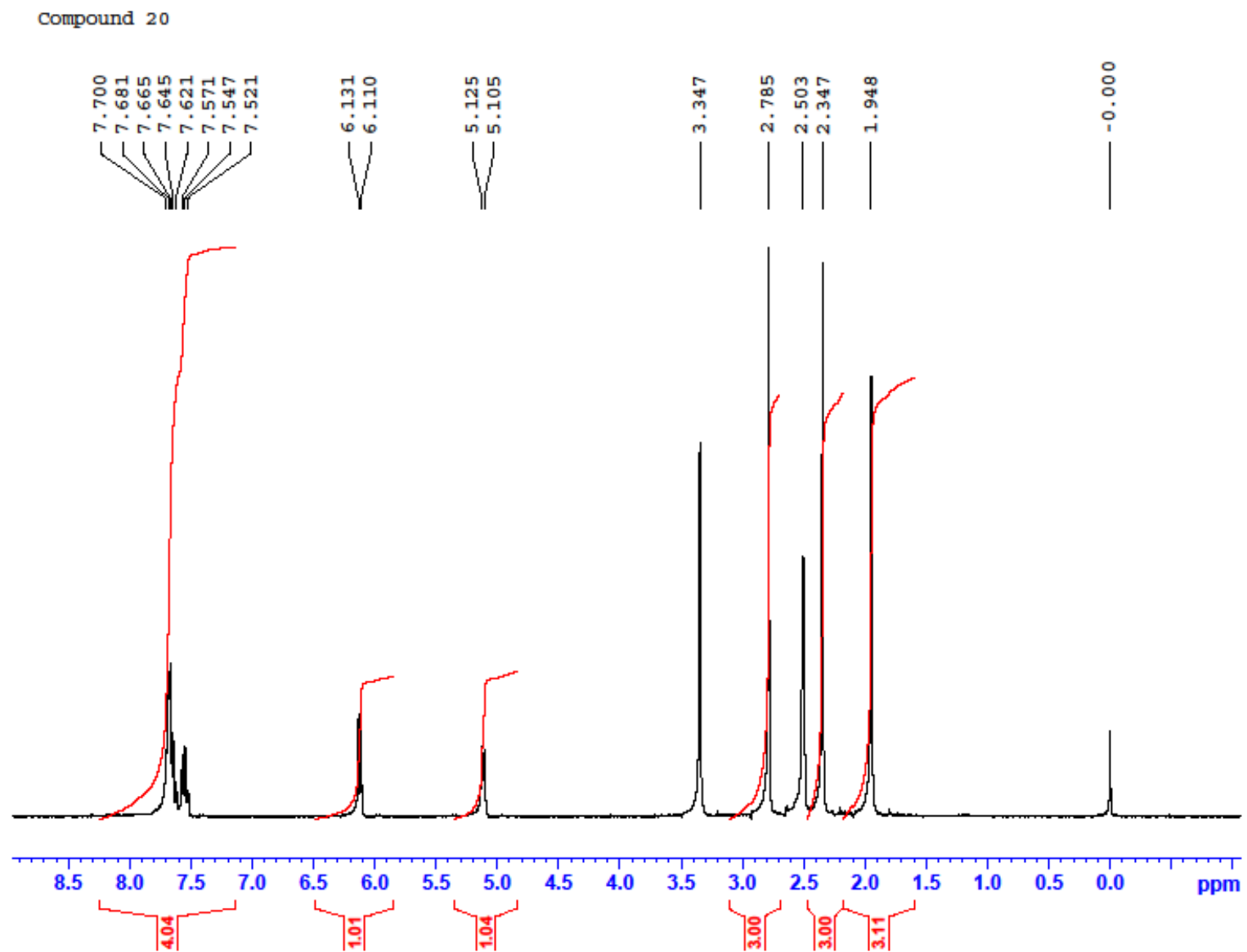
Figure S3. ^1\text{H-NMR} spectrum of compounds 20.
