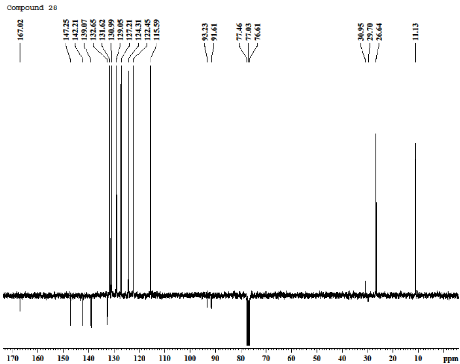
Figure S6. APT spectrum of compounds 28.
