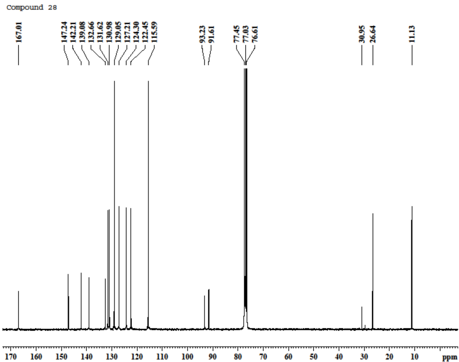
Figure S6. ^{13}\text{C} -NMR spectrum of compounds 28.
