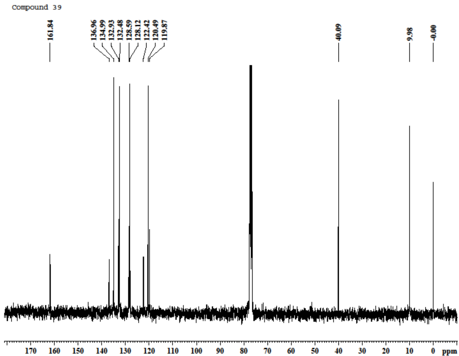
Figure S9. ^{13}\text{C} -NMR spectrum of compounds 39.
