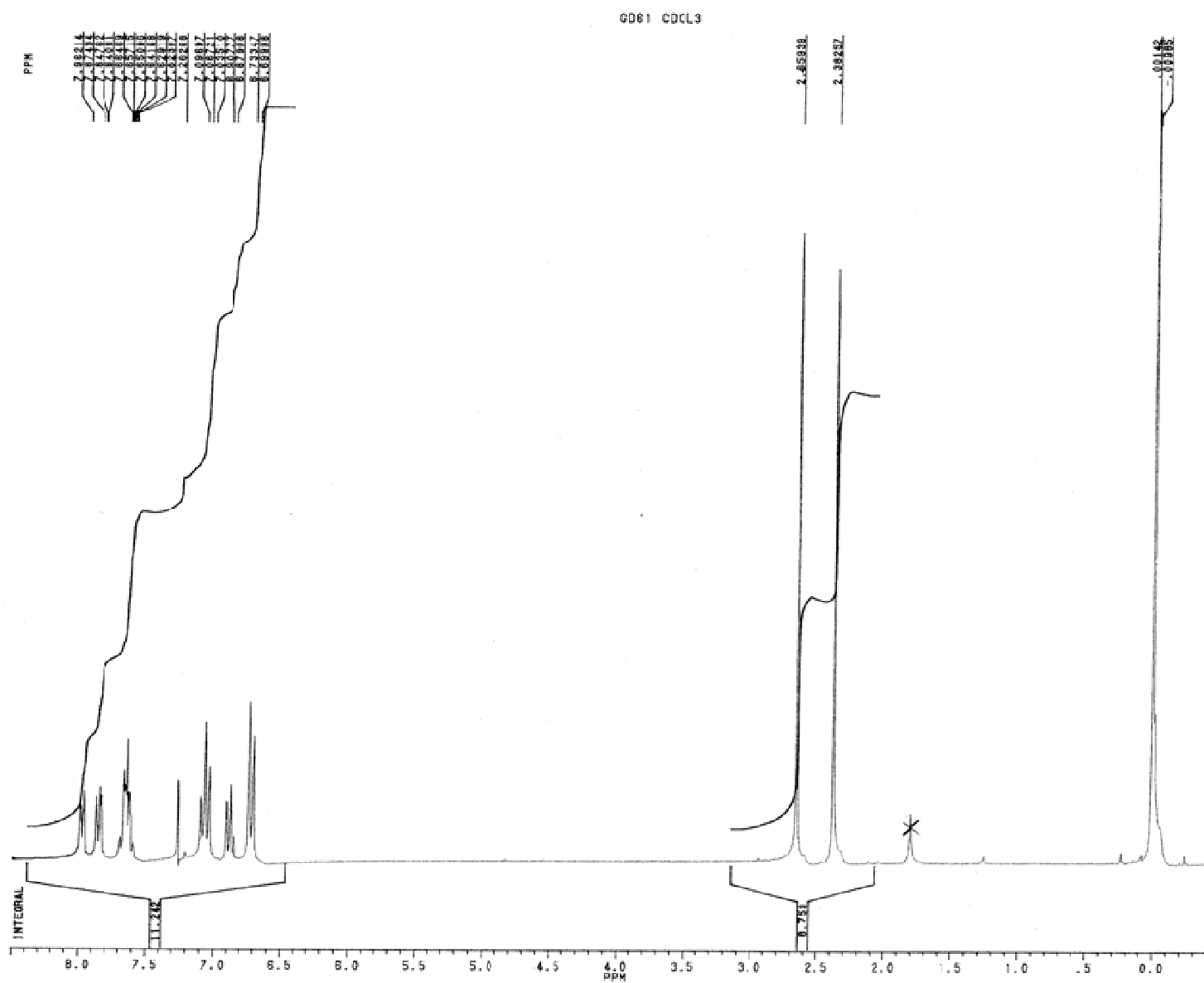
Figure S7. ^1\text{H-NMR} spectrum of compounds 29.
