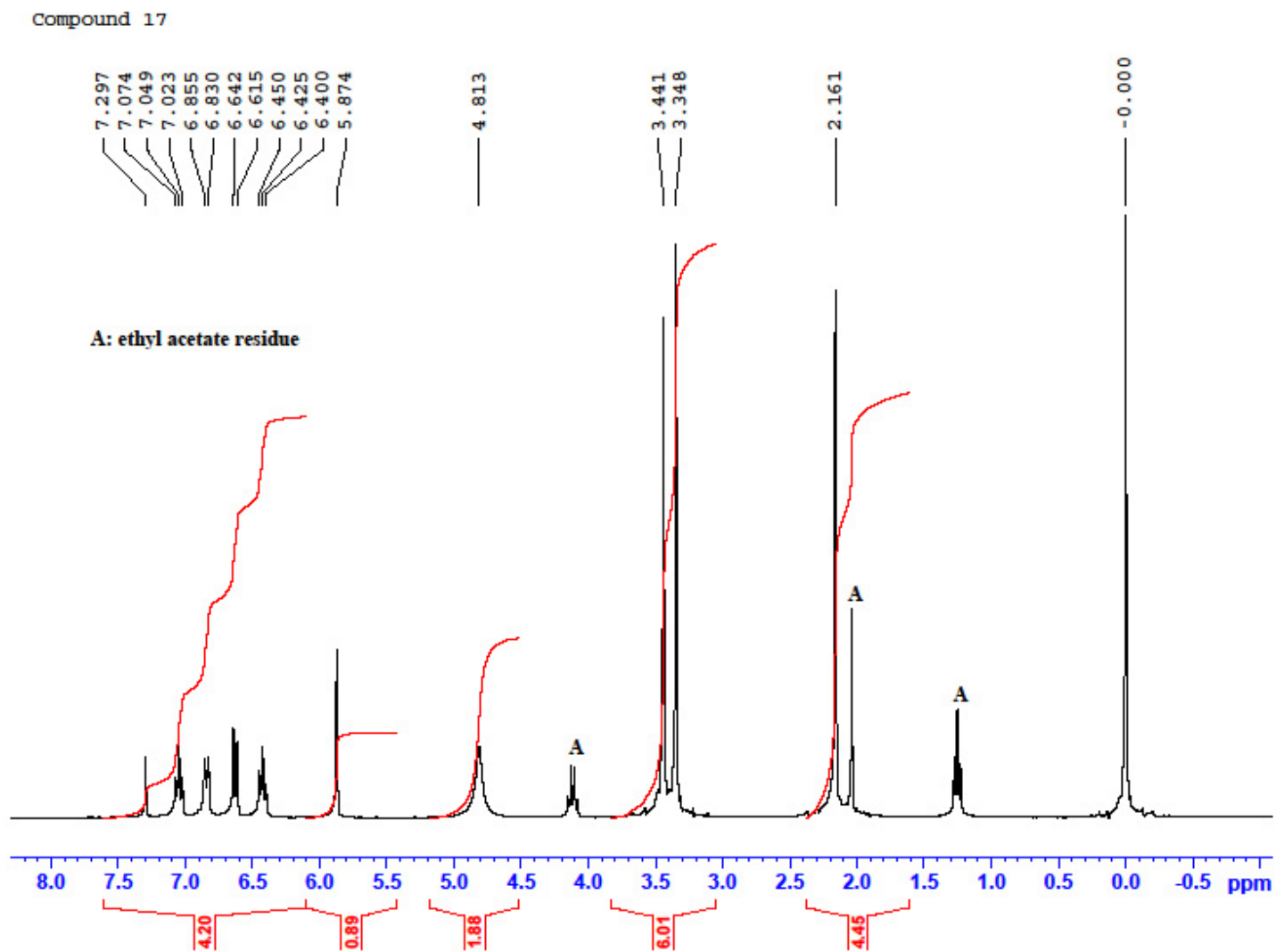
Figure S1. ^1\text{H-NMR} spectrum of compounds 17.
