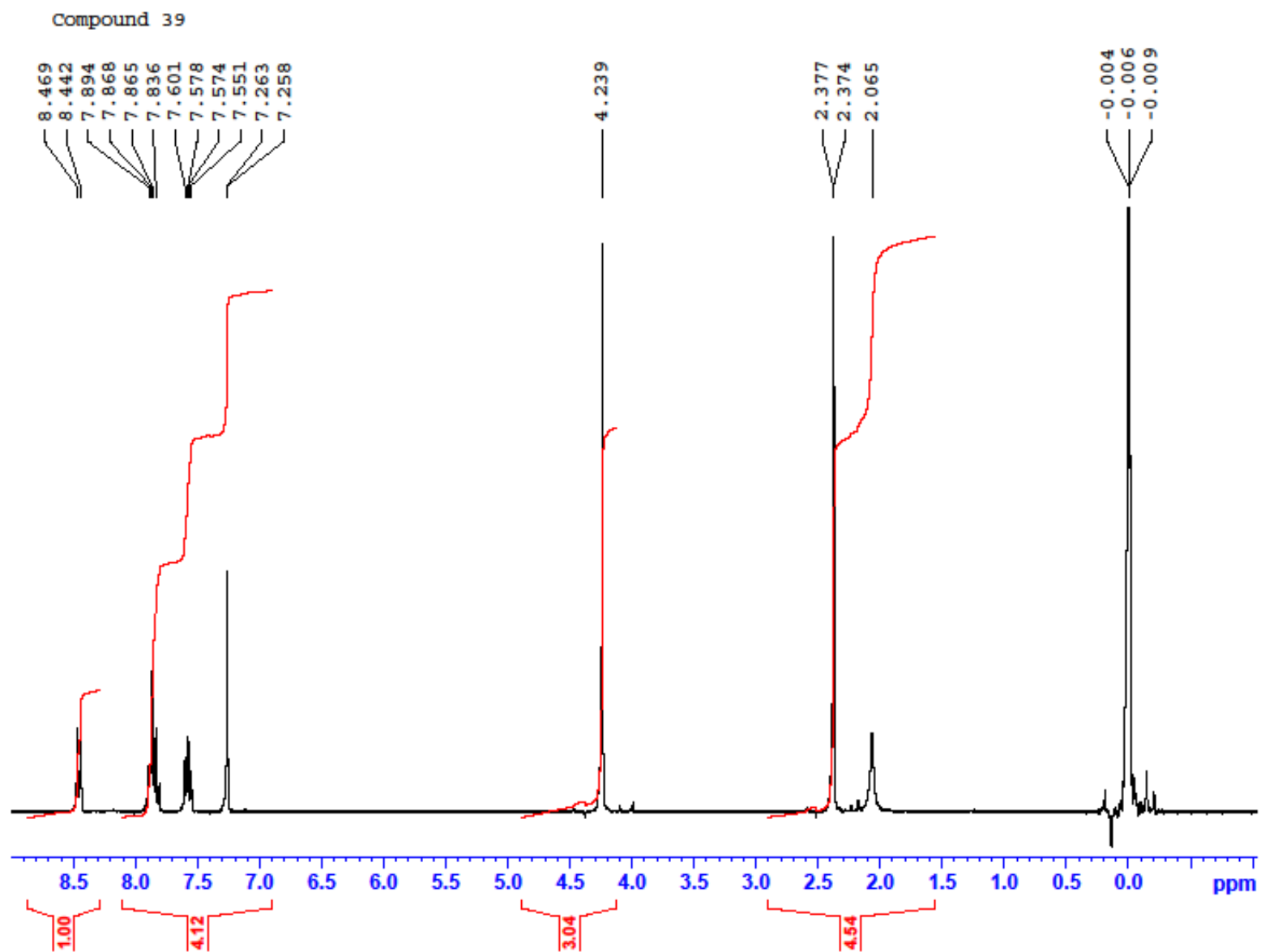
Figure S8. ^1\text{H-NMR} spectrum of compounds 39.
