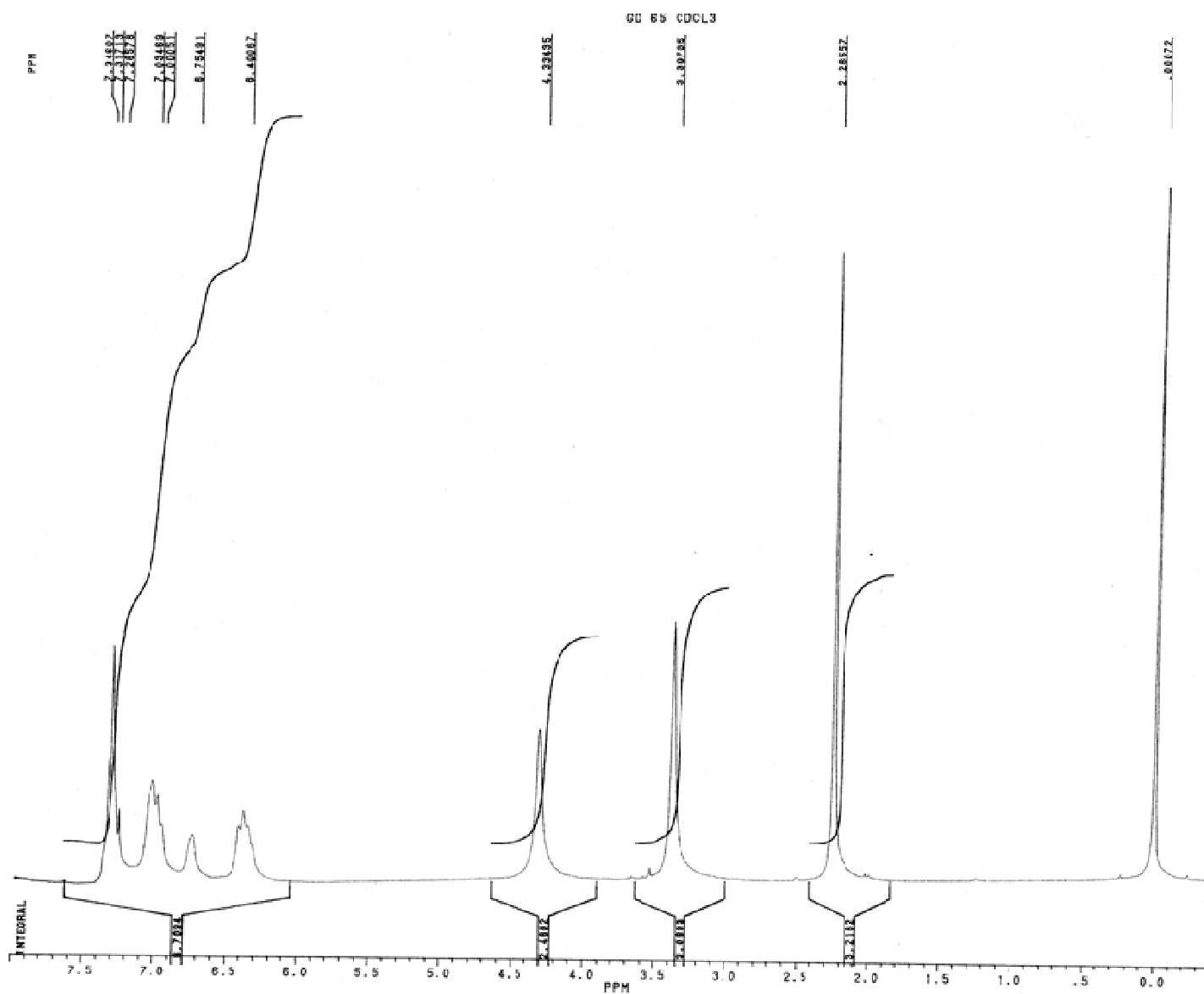
Figure S5. ^1\text{H-NMR} spectrum of compounds 28 .
