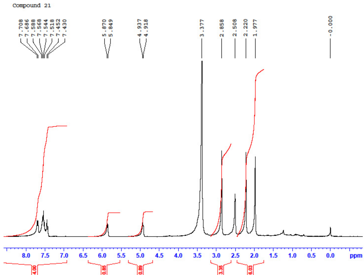
Figure S4. ^1\text{H-NMR} spectrum of compounds 21.
