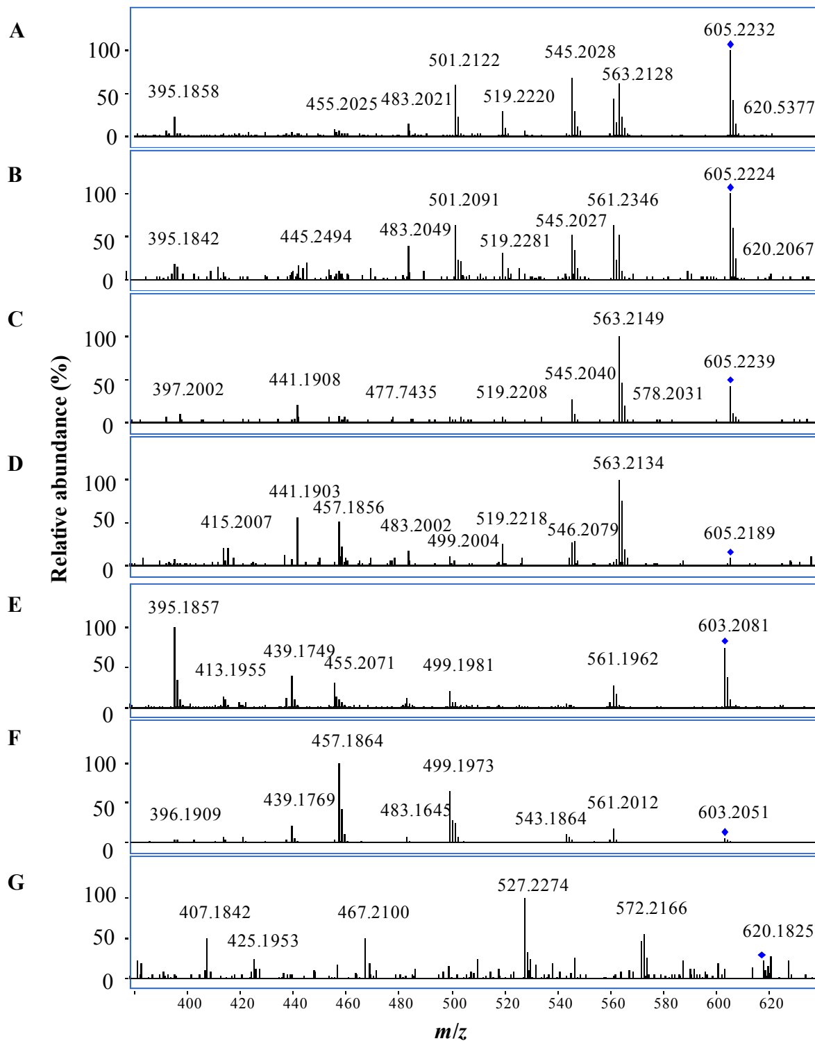
Figure S3. MS/MS spectra of metabolites in vitro , M1 (A), M2 (B), M3 (C), M4 (E), M5 (F), and M6 (G) at CE of 20 eV and M3 at CE of 30 eV (D).
