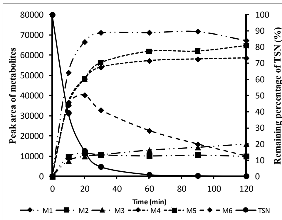
Figure S2. Amount-time relationship of toosendanin (TSN) and its six metabolites in vitro .
