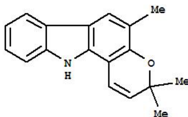
Figure 1. Structure of girinimbine (3,3,5-trimethyl-11H-pyrano[3,2-a]carbazole).
