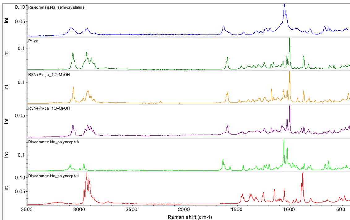
Figure 14. FT-Raman spectra of semi-crystalline risedronate monosodium salt (RSN), forms A and H, phenyl- \beta -D-galactopyranoside (Ph-gal) and samples 6 and 7 .
