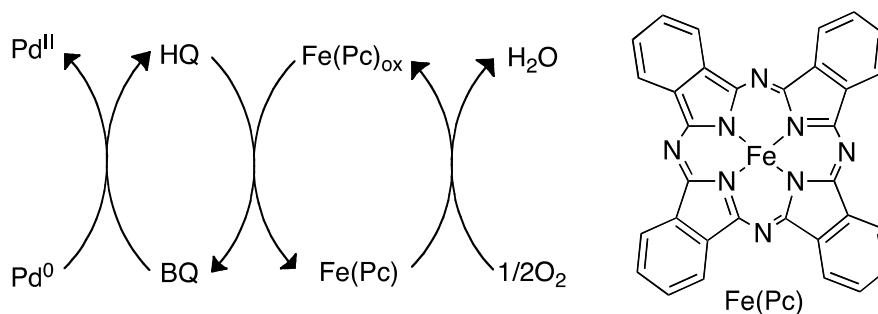
Scheme 17. Reoxidation of Pd 0 by use of BQ, iron and O 2 [80].
