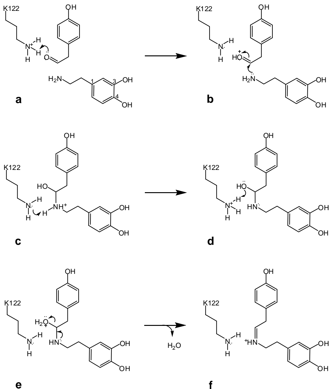
Scheme 2. Mechanism of NCS catalyzed iminium ion formation as intermediate in (S)-norcoclaurine synthesis.
