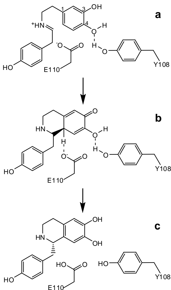
Scheme 3. Mechanism of NCS catalyzed synthesis of (S)-norcoclaurine.
