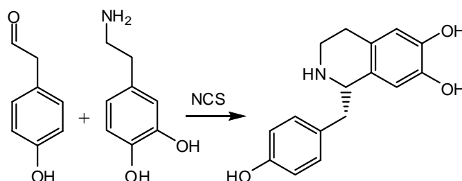
Scheme 1. ( S )-norcoclaurine biosynthesis.
