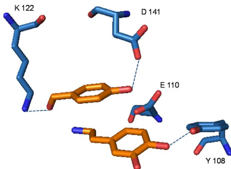
Figure 1. Amino acid residues involved in NCS catalysis.
