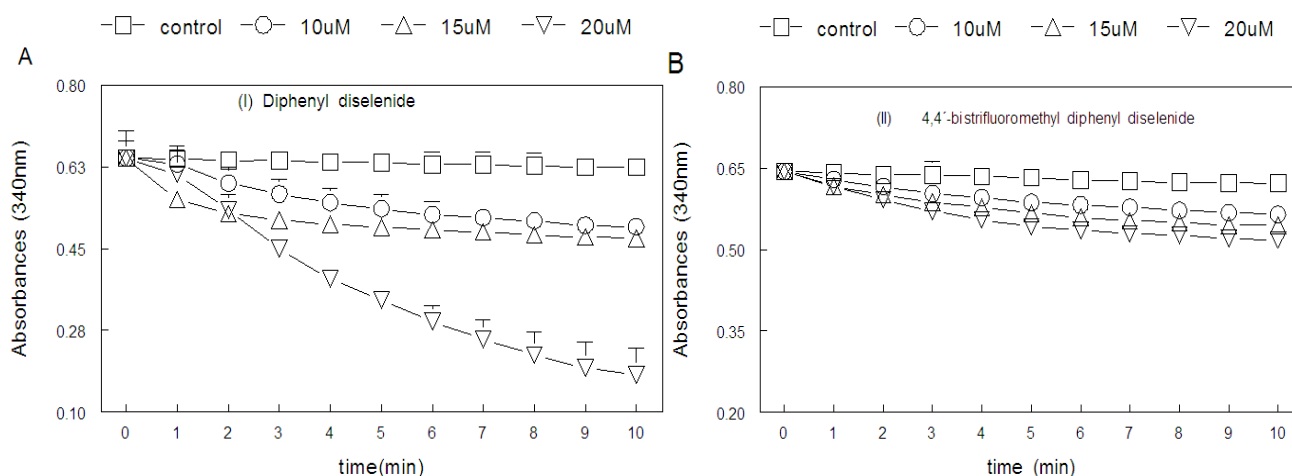
Figure 2. Reduction of diselenide compounds I (A), II (B), III (C), IV (D), V (E) e VI (F) by NADPH catalyzed by mammalian Thioredoxin Reductase (TrxR). Enzyme was mixed with a medium containing 50 mM Tris-HCl, 1 mM EDTA, pH 7,5 and then reaction was started by adding NADPH (final concentration 100 \mu\text{M} ). 0 ( \square ), 10(O), 15( \Delta ), 20( \nabla ) \mu\text{M} diselenide compounds. Statistical analysis were performed by three-way ANOVA (six diselenides \times four concentrations \times 11 sampling points). Data analysis yielded a significant diselenide \times concentration \times time interaction F(150, 1,440) = 42.5 ; p < 0.000001 , which indicates that the consumption of NADPH was dependent on the concentration, on the type of compound and on the sampling time.
