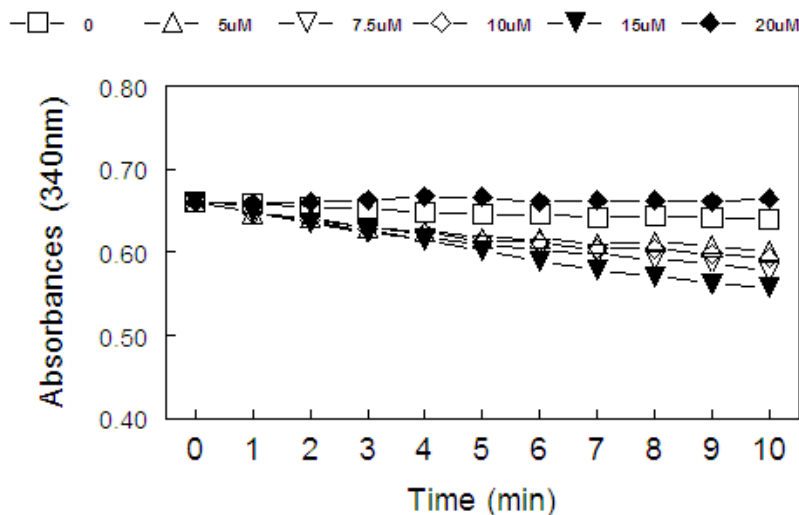
Figure 3. Reduction of ebselen (0, 5, 7.5, 10, 15 or 20 \mu\text{M} ) by NADPH catalyzed by mammalian TrxR. Enzyme was mixed with a medium containing 50 mM Tris-HCl, 1 mM EDTA, pH 7.5 and, then reaction was started by adding NADPH (final concentration 100 \mu\text{M} ). Statistical analysis were performed by two-way ANOVA (six concentrations \times 11 time points). Data analysis yielded a significant concentration \times time interaction [F(50, 360) = 24.6; p < 0.000001 ], which indicates that the consumption of NADPH determined in the presence of ebselen depended both on its concentration and on time of sampling.
