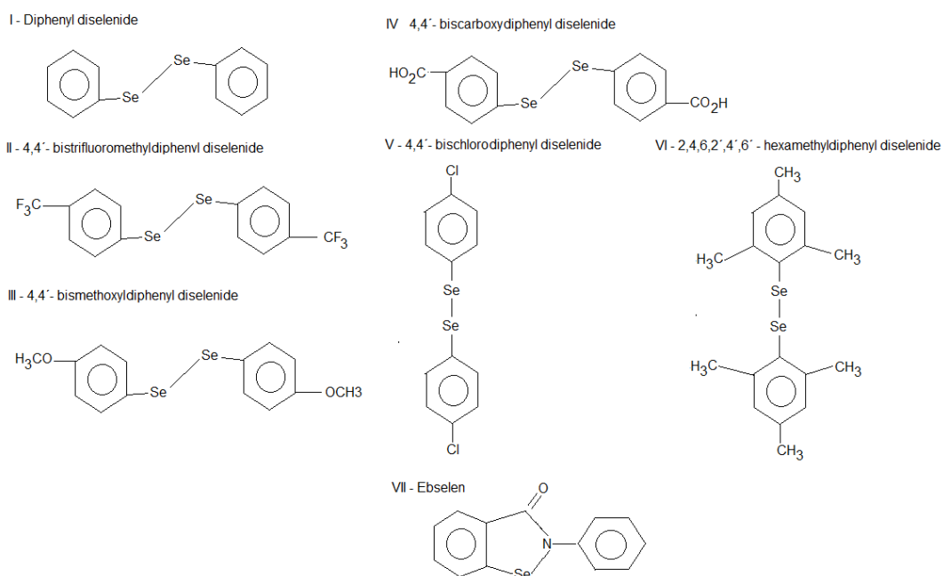
Figure 1. Structures of diselenide compounds.
