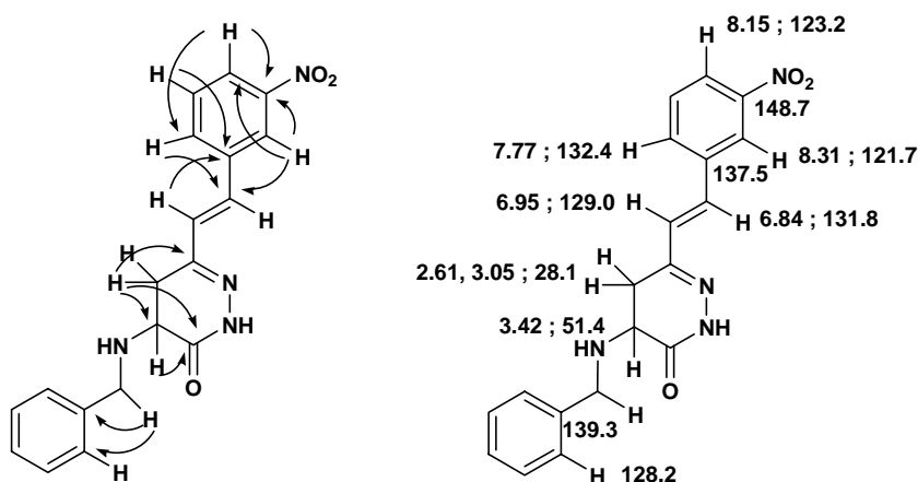
Scheme 6. Important connectivities found in the HMBC spectra of 15 , and ^1\text{H} - and ^{13}\text{C} -NMR assignments.
