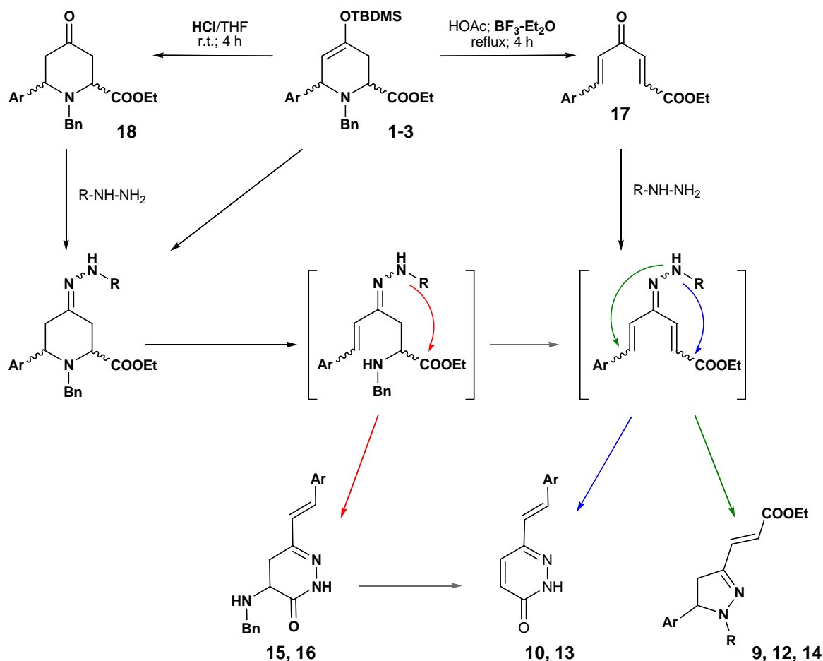
Scheme 8. Proposal for the formation of pyrazolines and pyridazinones.
