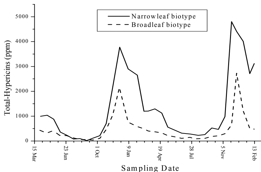
Figure 1. Seasonal variation in hypericin concentrations in Australian St John's Wort
