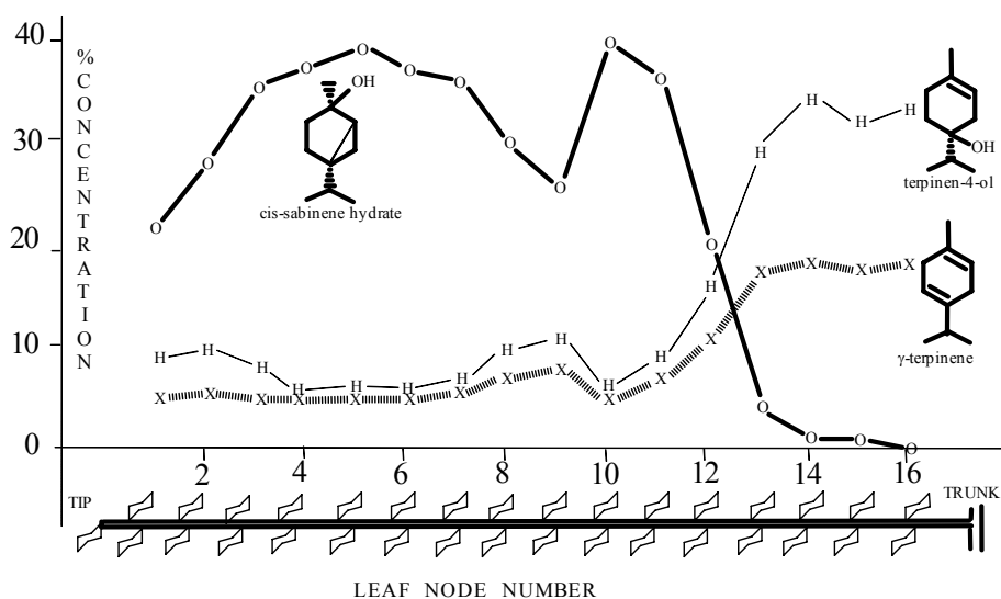
Figure 2. Along the branch variation in the concentrations of cis -sabinene hydrate, terpinen-4-ol and \gamma -terpinene in individual leaves of M. alternifolia .
