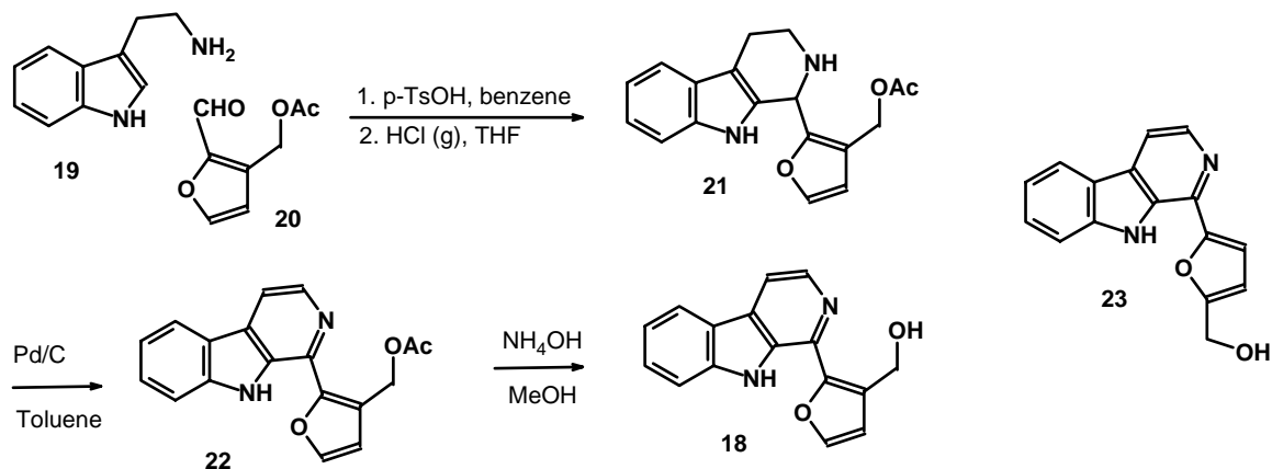
Scheme 1. The Synthesis of Tribulusterine
