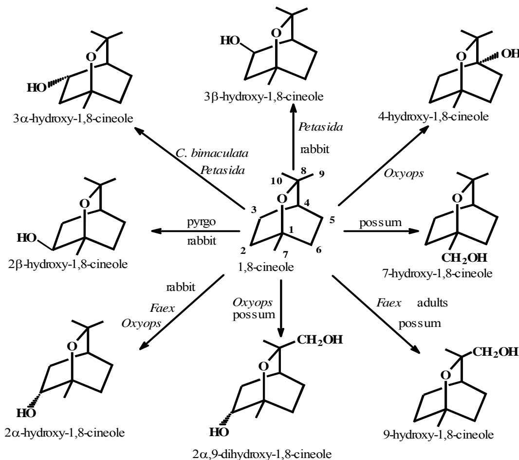
Figure 4. Metabolism of 1,8-cineole by a variety of insects (pyrgo, Chrysophtharta bimaculata , Petasida , Oxyops , Faex ) and mammals (rabbit, possum).
