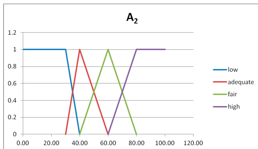
Figure 5. Graph of the fuzzy sets of the fuzzy partition for U_{x2} .
