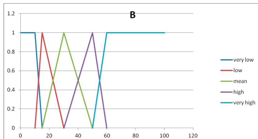
Figure 6. Graph of the fuzzy sets of the fuzzy partition for U_y .
