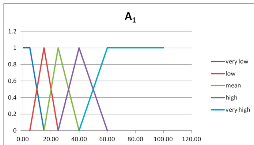
Figure 4. Graph of the fuzzy sets of the fuzzy partition for U_{x1} .
