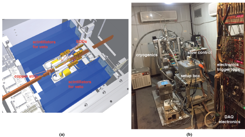
Figure 1. (a) The design of the core components of the Violation of Pauli exclusion principle 2 (VIP-2) setup, including the silicon drift detectors (SDDs) as the X-ray detector, the scintillators as active shielding with silicon photomultiplier readout; (b) a picture of the VIP-2 setup in operation at the underground laboratory of Gran Sasso.
